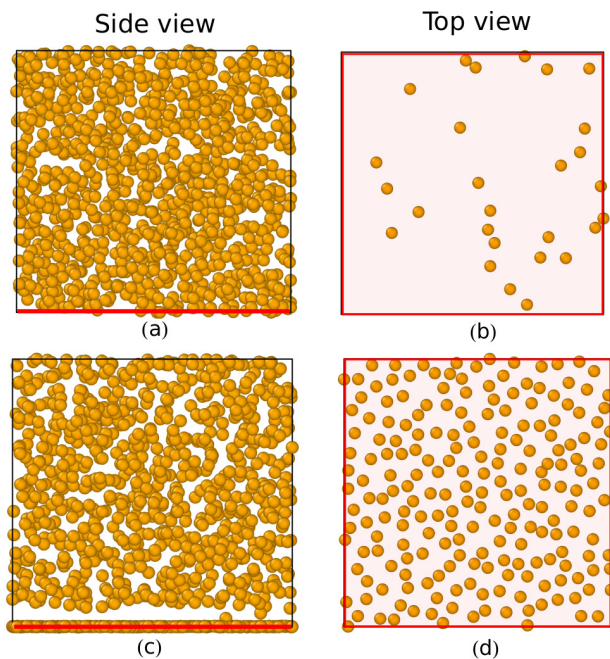
Figure 7: Snapshots of Brownian dynamics simulations used to analyze the adsorption of silica nanoparticles onto alumina. Initial conditions: (a) picture of the box and (b) sliced view of the bottom wall. Results of simulations at t = 0.0075 s: (c) picture of the box and (d) sliced view of the bottom wall.
