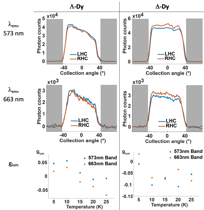
Figure S9. Angular distribution of the emission (bands at 573-nm and 663-nm) recorded at 5K, and temperature dependent variation of the dissymmetry factor g_{lum} for a crystalline powder of (left) \Lambda -Dy and (right) a \Delta -Dy crystal. The grey portions correspond to the angles not collected by the objective (outside the numerical aperture).
