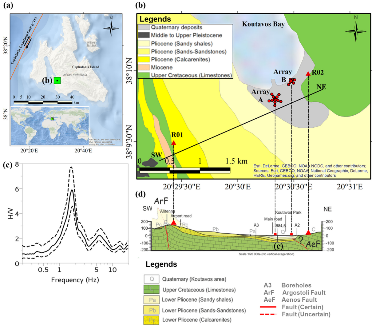
Figure 1. (a) The Argostoli study area, marked by the green rectangle, on the island of Cephallonia. (b) Zoomed view on the geological map of Argostoli (Cushing et al. 2016, 2020) along with the locations of Array A, Array B and the nearby rock stations (R01, R02). (c) H/V average spectral ratios ( \pm 1\sigma ) at the centre of the valley from 1 hr of ambient noise recordings.
