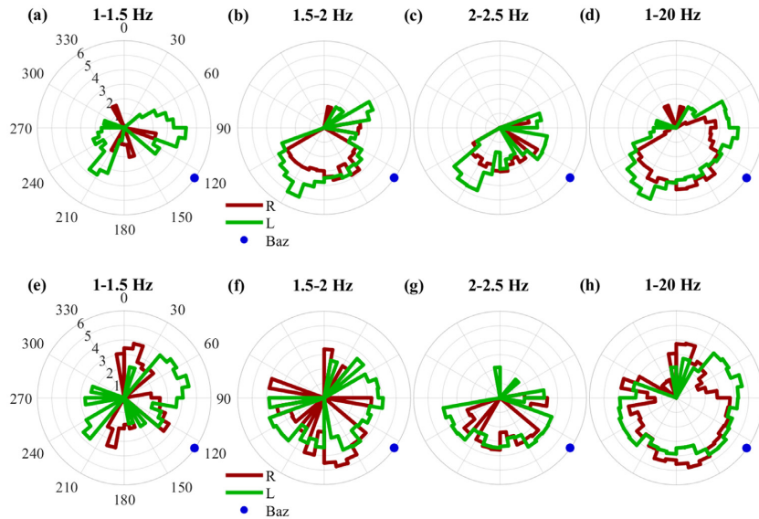
Figure 10. Polar distribution of the Love (L) and Rayleigh (R) wave energies for the different 10 degree intervals in different frequency ranges for (a)–(d) Array A and (e)–(h) Array B data from event no. 12. The blue dot indicates the backazimuth (Baz) of the event.
