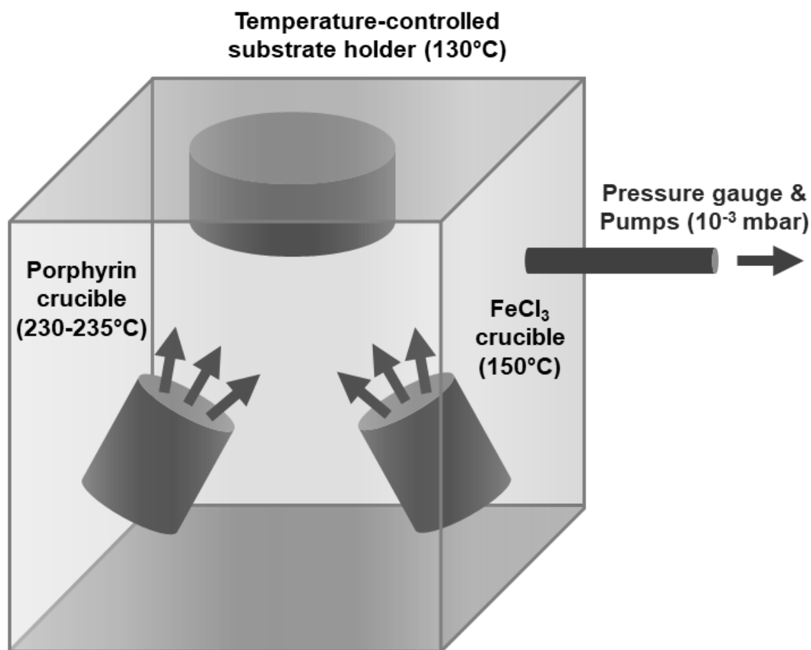
Scheme S1. Oxidative chemical vapour deposition (oCVD) reactor used for the preparation of the pNiDPP and pNiDMP thin films and CuPc/pNiDPP, Cu(F 16 Pc)/pNiDPP, CuPc/pNiDMP and Cu(F 16 Pc)/pNiDMP devices. The nickel(II) porphyrins (NiDPP and NiDMP) and the oxidant (FeCl 3 ) were simultaneously sublimed under reduced pressure ( 10^{-3} mbar) using two crucibles located in the lower part of the chamber. The crucible temperatures were set to 235°C, 230°C and 150°C for NiDPP, NiDMP and FeCl 3 , respectively. The substrates were placed on a heated stage (130°C) placed 20 cm above the two crucibles. The reference sNiDPP and sNiDMP thin films were prepared by sublimation using the same chamber without FeCl 3 .
