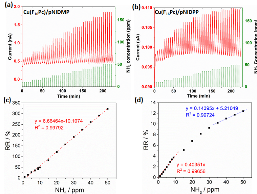
Figure 7. Current variations of Cu(F 16 Pc)/pNiDMP (a) and Cu(F 16 Pc)/pNiDPP (b) devices submitted to \text{NH}_3 in the range 10–50 ppm, by steps of 5 ppm, during alternate exposure/recovery cycles (1 min/4 min), at 40% rh. RR variation as a function of \text{NH}_3 concentration in 1–50 ppm range, in air, at 40% rh, during exposure/recovery cycles (1 min/4 min) of Cu(F 16 Pc)/pNiDMP (c) and Cu(F 16 Pc)/pNiDPP (d) devices.
