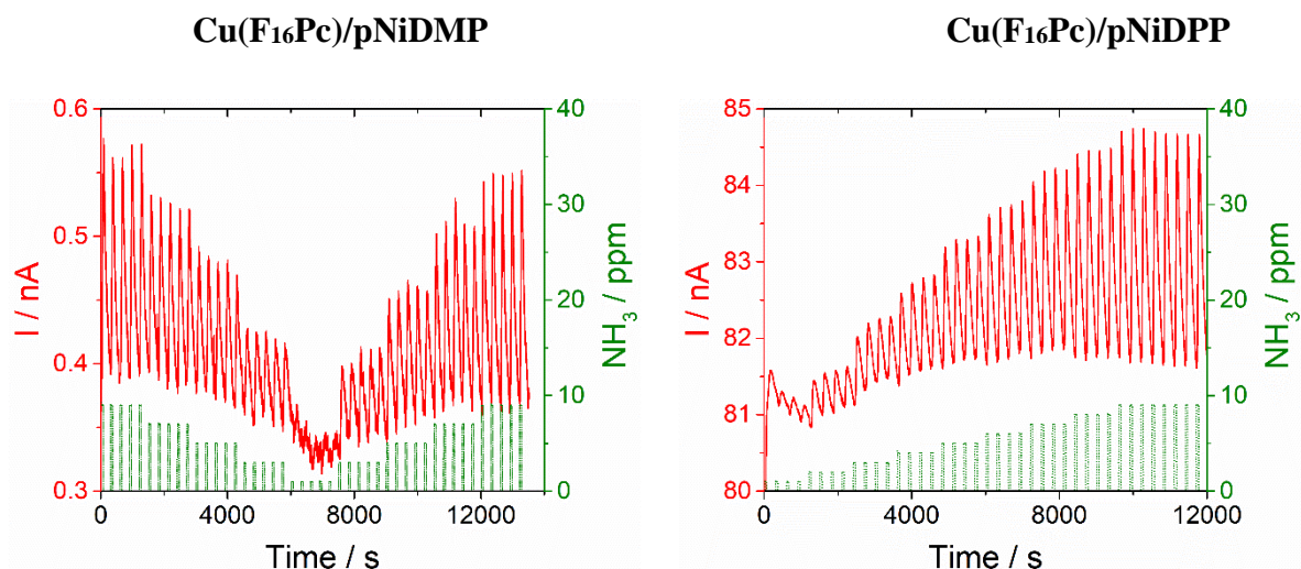
Figure S8. Response of Cu(F 16 Pc)/pNiDMP (left, at a bias of 2 V) and Cu(F 16 Pc)/pNiDPP (right, at a bias of 5 V, to NH 3 , in the range 1-9 ppm, during exposure/recovery cycles (1 min / 4 min), at 40 % RH.
