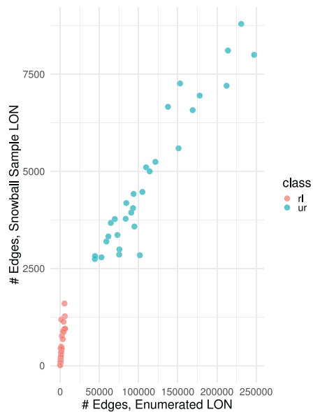
(b) Comparing LON edge (optima connections) counts
