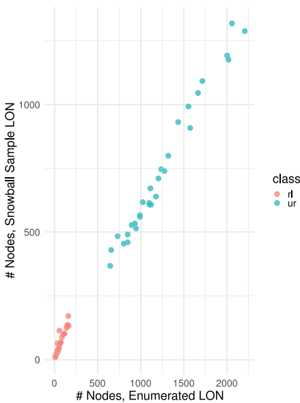
(a) Comparing LON node (local optima) counts
