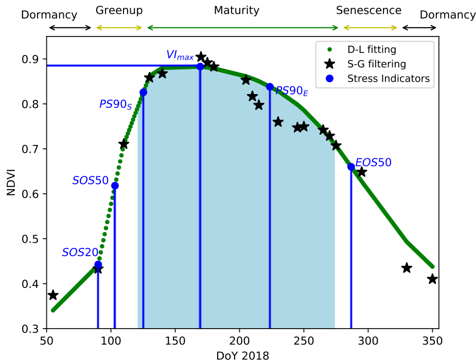
Figure 4. Phenological curve as described by Normalized Difference Vegetation Index (NDVI) (Double logistic approximation in green and Savitzky–Golay filtering in black) and annual phenological characterization criteria (blue), Green period area is colored in light blue for clarity. Case study of Canal de Brienne area, Toulouse, 2018. Main vegetation phenological periods are outlined in the top of the figure: Dormancy, Greenup, Maturity and Senescence [44].
