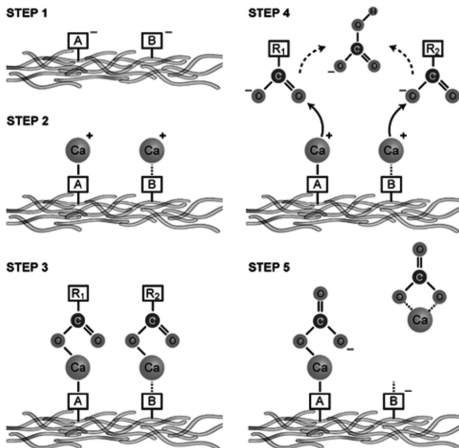
Figure 12. Conceptual model of calcium carbonate precipitation in the biofilm from Braissant et al. (2009). Step 1: EPS functional groups (A and B); step 2: calcium binding more or less tightly to functional groups A and B; step 3: complex formation between LMW organic carbon compound and calcium; step 4: release of LMW organic carbon by microbial activity and oxidation to HCO 3 - which in turn increases TA within the biofilm; step 5: CaCO 3 formation either on EPS or in pockets within the biofilm. Permission of Federation of European Microbiological Societies.
