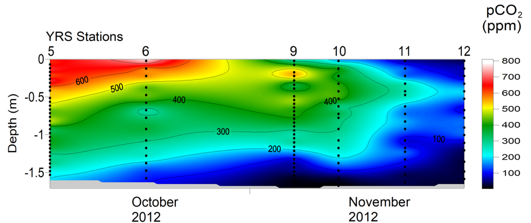
Figure 9. Temporal evolution of pCO 2 . Samples were analyzed with a standard gas of 300 ppm. Black dots are data points from field sampling. This plot was produced using the radial basis function method for interpolation in Surfer 8 software.
