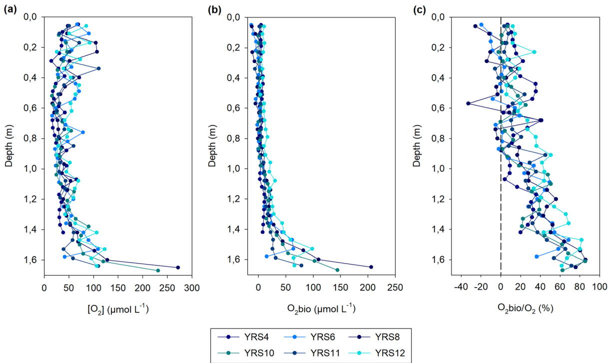
Figure 8. Vertical profiles of (a) O_2 concentrations in bulk ice, (b) [O_2]_{bio} calculated from Equation 5, and (c) O_2bio/O_2 ratio.
