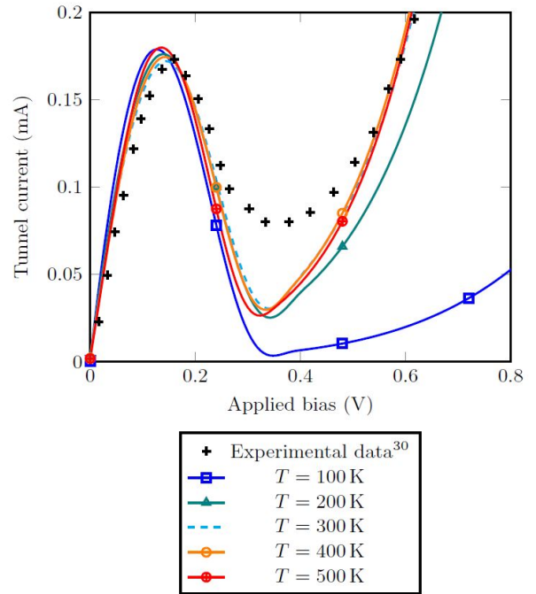
FIG. 7: Impact of temperature on a tunnel diode.
