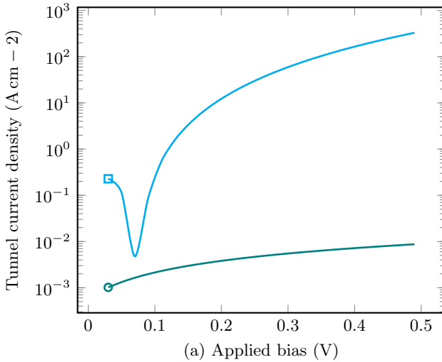
FIG. 1: Comparison of direct tunneling models at forward bias.
