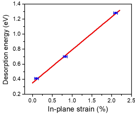
Figure 7: Desorption energy as a function of in-plane strain.
