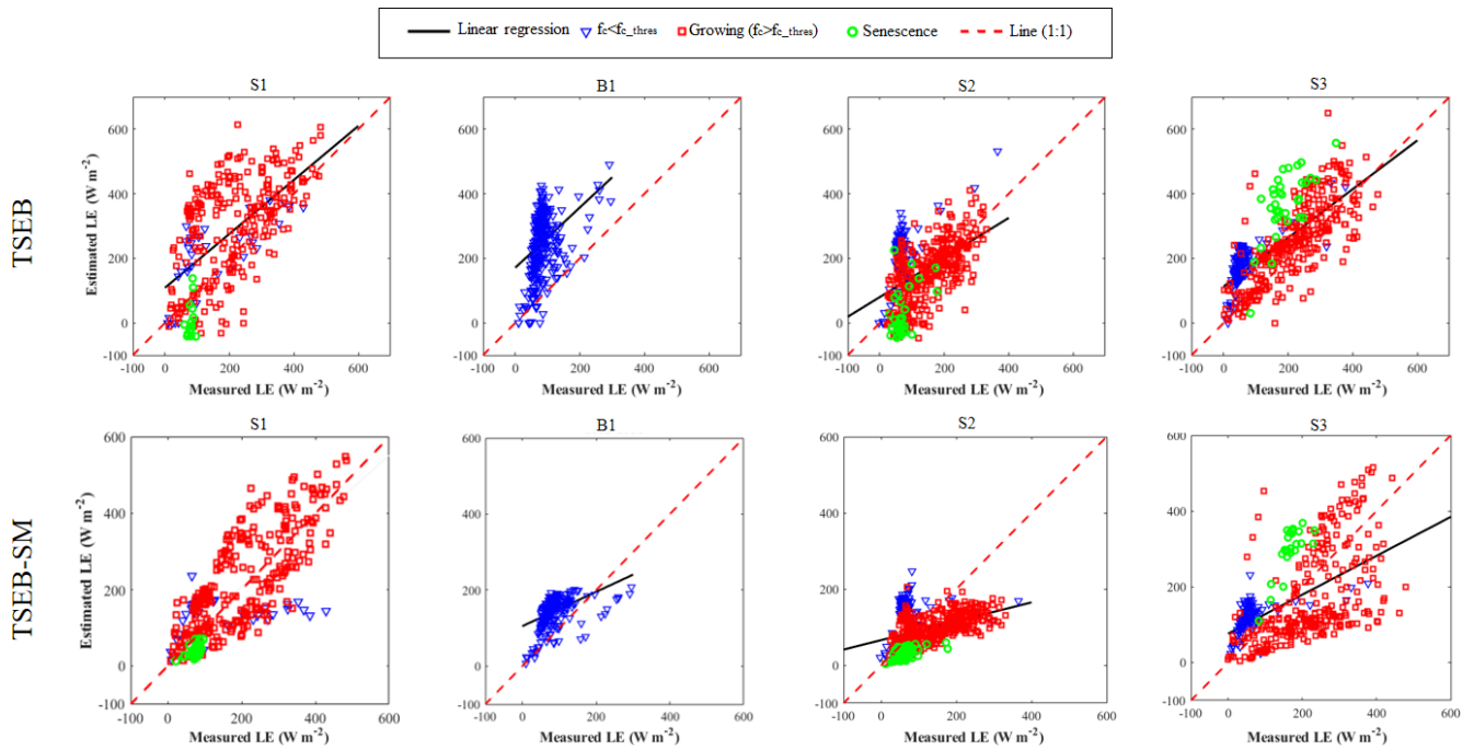
Figure 8. Scatterplot of simulated versus observed LE for (top panels) TSEB and (bottom panels) TSEB-SM models using in situ data collected during S1, B1, S2 and S3, respectively.
