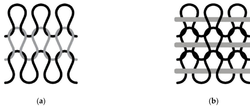
Figure 1. (a) Example of a knitted structure with loops (single jersey); and (b) the same knitted structure with an inlay yarn (the ground yarn making loops is shown in black and the inlay yarn in grey).
