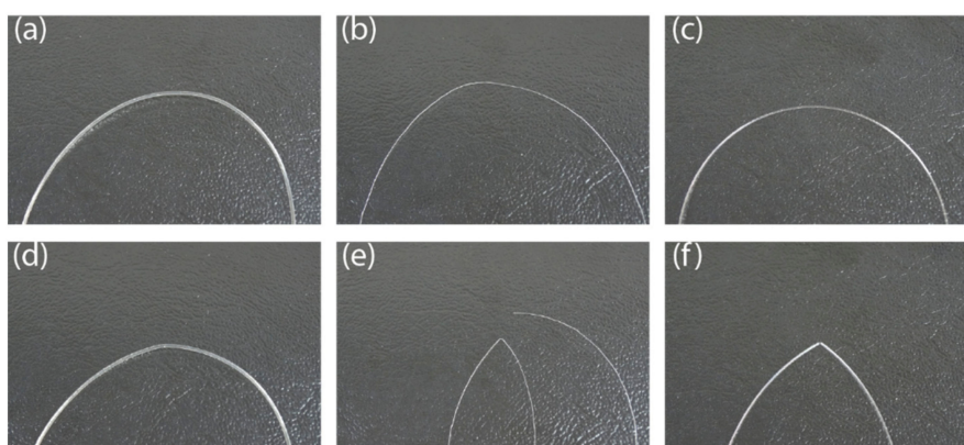
Figure 5. Evaluation of the plastic behavior of optical fibers under bending, with a radius of 1 mm: Empa Geniomer ® (a) before testing and (d) 2 min after testing; Empa bi-component (b) before testing and (e) 2 min after testing; GigaPOF 50-SR (c) before testing and (f) 2 min after testing.
