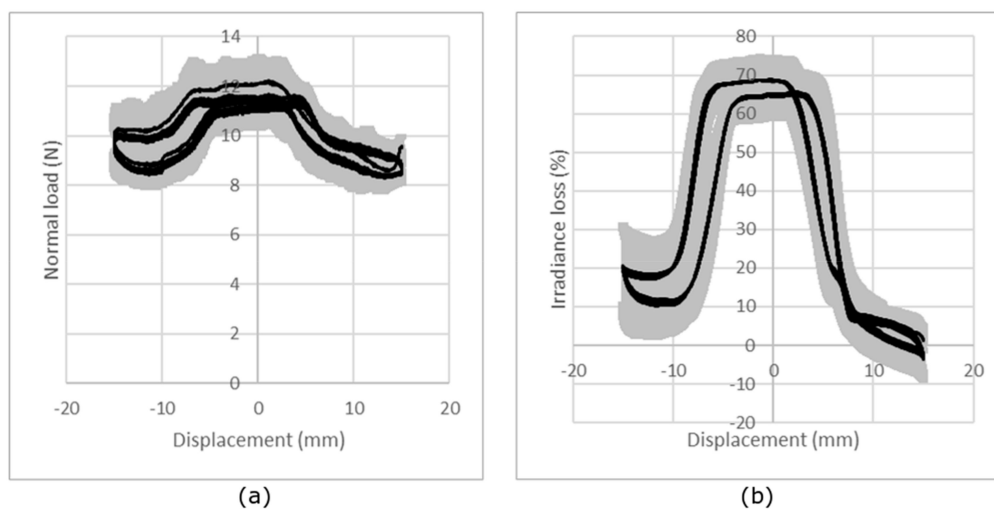
Figure 11. Reproducibility of measurements: (a) evolution of the normal force and (b) evolution of the loss of irradiance relative to the displacement of the slider for five samples of single jersey under a nominal load of 10 N. The black line represents the average curve and the gray area the standard deviation.
