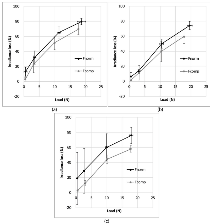
Figure 16. Comparison between the evolution of the irradiance loss as a function of the normal load during friction ( F_{norm} ) or compression tests ( F_{comp} ) for (a) single jersey; (b) 1 \times 1 rib; (c) 1 \times 1 interlock, with the error bars representing the standard deviation.
