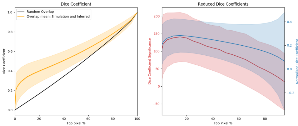
Fig. 13. Left: dice coefficient (as defined by Eq. (9)) of the top n\% voxels between the 3D simulation cubes and their inferred counterparts in increments of 5% (yellow). The inner dark yellow layer represents the measure uncertainty, and the outer yellow layer represents the standard deviation over the set. The random overlap is represented in black. Right, red: dice coefficient significance (see Eq. (11)). Blue: Normalized Dice coefficient (see Eq. (10)). The coefficients are represented with their standard deviation layers.
