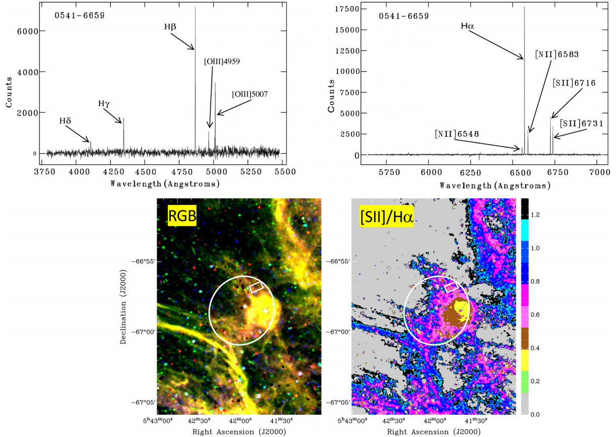
Figure A16. MGSNR J0541–6659: (Top) showing the spectra from both arms (left-hand panel; blue, right-hand panel; red) of the spectrograph; (Bottom) colour images produced from MCELS data, where RGB corresponds to H\alpha , [S II], and [O III] while the ratio map is between [S II] and H\alpha . The rectangular box (white) represents an approximate position of the WiFeS slicer. The white circle indicates the location of the optical shell.
