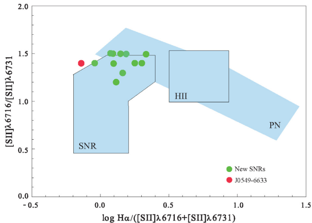
Figure 2. Ratio of [S II]\lambda 6716 and [S II]\lambda 6731 lines versus \log H\alpha/([S II]\lambda 6716 + [S II]\lambda 6731) for the sample of our 12 spectroscopically observed LMC objects presented in this paper. 11 objects from Table 2 fit in the designated area of SNRs while the object marked as a red dot (J0549–6633; Section A19) is slightly out. Noticeably, all these objects occupy the area suggested for older remnants as predicted by Sabbadin et al. (1977).
