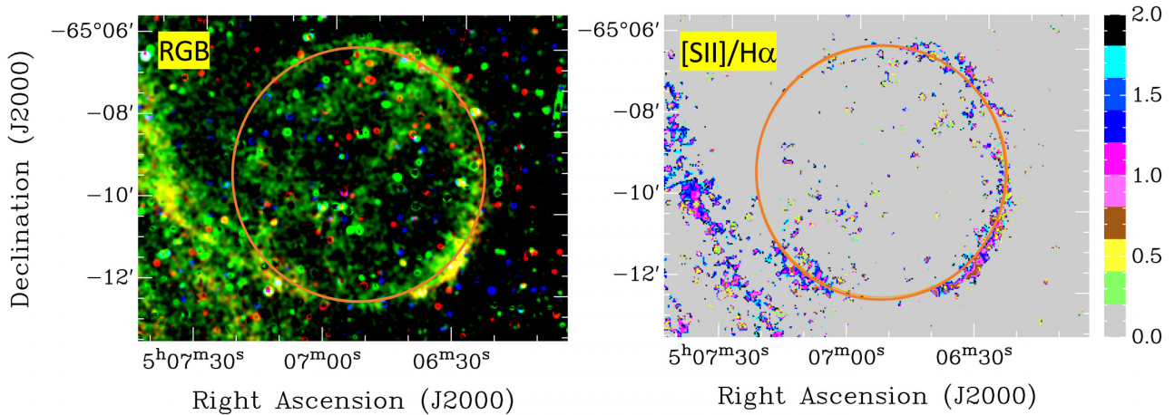
Figure A7. J0506–6509: colour images produced from MCELS data, where RGB corresponds to H\alpha , [S II] , and [O III] while the ratio map is between [S II] and H\alpha . The orange circle indicates the extent of the optical emission seen from the object.
