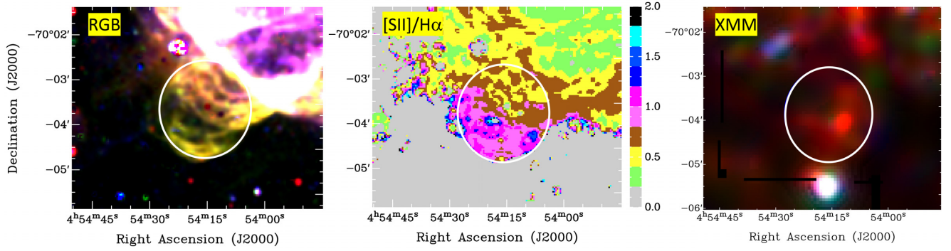
Figure A3. J0454–7003: colour images produced from MCELS data, where RGB corresponds to H\alpha , [S\ II] , and [O\ III] (left-hand panel) while the ratio map is between [S\ II] and H\alpha (middle). XMM-Newton EPIC RGB ( R = 0.3\text{--}0.7\text{ keV} band, G = 0.7\text{--}1.1\text{ keV} band and B = 1.1\text{--}4.2\text{ keV} band) image from the area of J0454–7003 is shown in the right-hand panel. The white circle indicates the extent of the optical emission seen from the object. The line-shaped features in the left-hand and bottom hand side of the image are smoothing artefacts, caused by borders of adjacent observations, which introduce steps in exposure.
