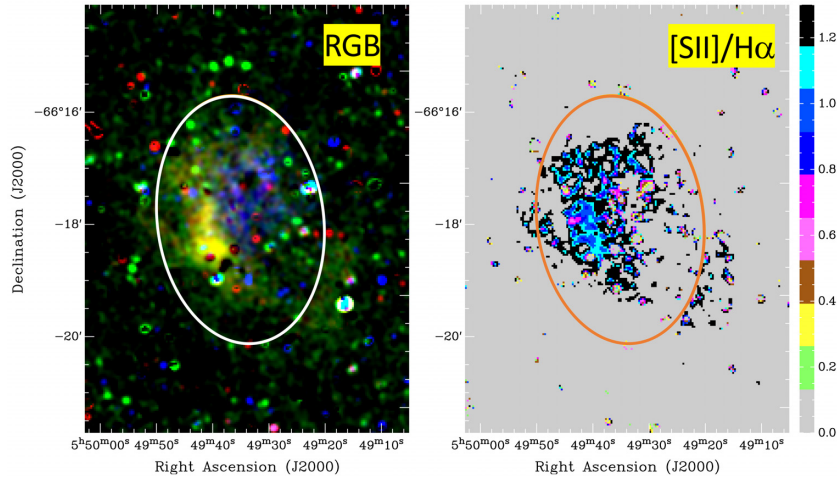
Figure A20. J0549–6618: colour images produced from MCELS data, where RGB corresponds to H\alpha , [S\ II] , and [O\ III] while the ratio map is between [S\ II] and H\alpha . The white/orange ellipse indicates the location of the optical shell.
