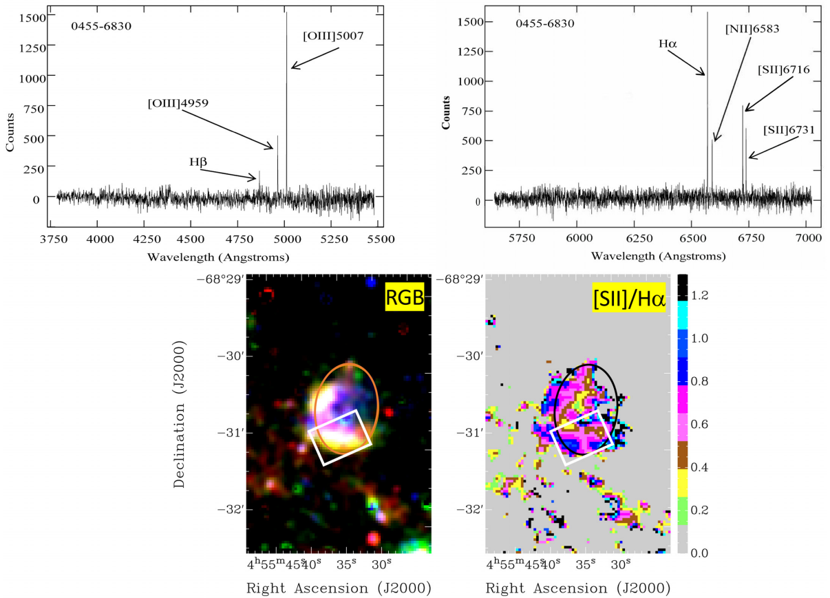
Figure A4. J0455–6830: (Top) showing the spectra from both arms (left-hand panel; blue, right-hand panel; red) of the spectrograph; (Bottom) colour images produced from MCELS data, where RGB corresponds to H\alpha , [S\ II] , and [O\ III] while the ratio map is between [S\ II] and H\alpha . The rectangular box (white) represents an approximate position of the WiFeS slicer. The orange/black ellipse indicates the extent of the optical emission seen from the object.
