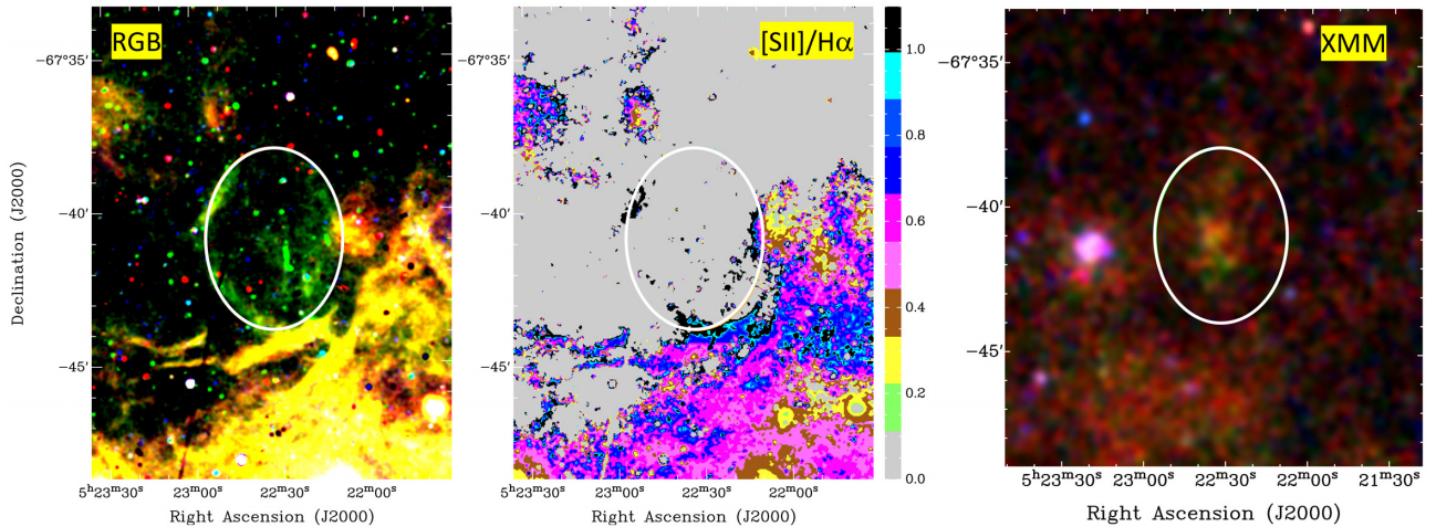
Figure A12. MCSNR J0522–6740: colour images produced from MCELS data, where RGB corresponds to H\alpha , [S\ II] , and [O\ III] (left-hand panel) while the ratio map is between [S\ II] and H\alpha (middle). XMM-Newton EPIC RGB ( R = 0.3\text{--}0.7 keV band, G = 0.7\text{--}1.1 keV band and B = 1.1\text{--}4.2 keV band) image from the area of MCSNR J0522–6740 is shown in the right-hand panel. The white ellipse indicates the location of the optical shell.
