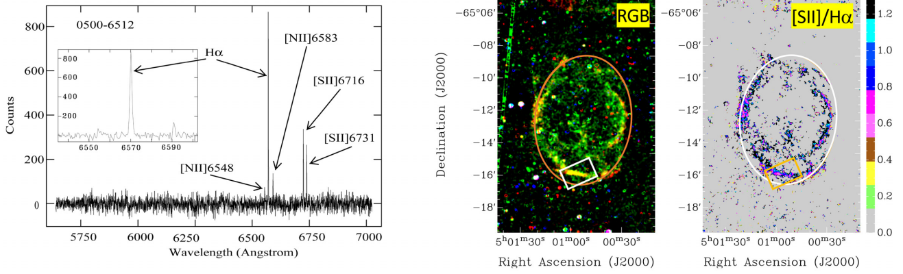
Figure A5. J0500–6512: (Left-hand panel) showing the spectra from one arm (red) of the spectrograph where the inset figure represents the ‘zoomed-in’ H \alpha line. This H \alpha line is detected with the broadening of 1.20 Å while the instrument width is \sim 1 Å ( \sim 45 km s ^{-1} ); (Middle and right-hand panel) colour images produced from MCELS data, where RGB corresponds to H \alpha , [S II], and [O III] while the ratio map is between [S II] and H \alpha . The rectangular box (white/orange) represents an approximate position of the WiFeS slicer. The orange/white ellipse indicates the extent of the optical emission seen from the object.
