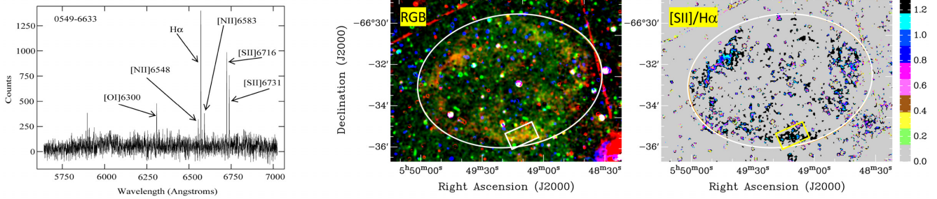
Figure A21. 0549–6633: (Left-hand panel) showing the spectra from one arm (red) of the spectrograph; (Middle and right) colour images produced from MCELS data, where RGB corresponds to H\alpha , [S\ II] , and [O\ III] while the ratio map is between [S\ II] and H\alpha . The rectangular box (white/yellow) represents an approximate position of the WiFeS slicer. The white ellipse indicates the location of the optical shell.
