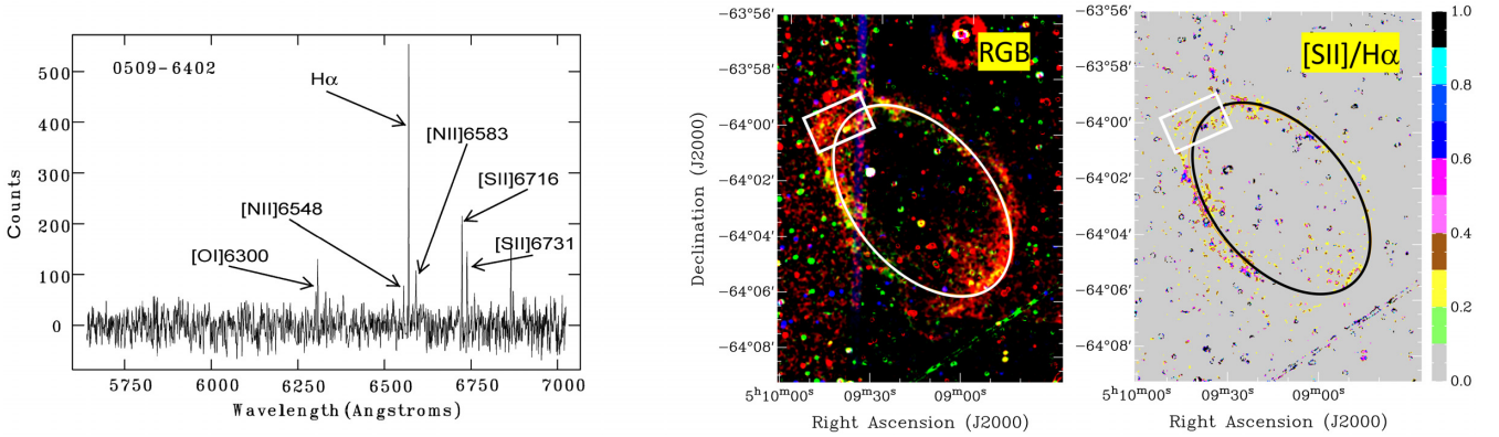
Figure A9. J0509–6402: (Left-hand panel) showing the spectra from one arm (red) of the spectrograph; (Middle and right) colour images produced from MCELS data, where RGB corresponds to H\alpha , [S\ II] , and [O\ III] while the ratio map is between [S\ II] and H\alpha . The rectangular box (white) represents an approximate position of the WiFeS slicer. The white/orange ellipse indicates the extent of the optical emission seen from the object.
