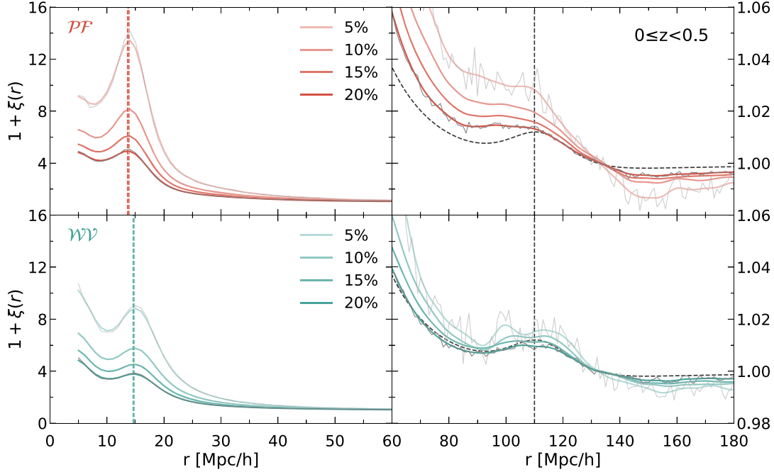
Figure 5. Same as Fig. 4, but for \mathcal{PF} (peak–filament) and \mathcal{WV} (wall–void) correlations in the top and bottom panels, respectively. For these cross-correlations, the vertical lines mark the positions of the maximum (left) and the BAO feature (right). We truncate the correlation function below r < 5 h^{-1} Mpc, since the pair counts at separation near the resolution scale ( \sim 2 h^{-1} Mpc) are numerically suppressed. The linear dark matter correlation function (dashed) at the median redshift of 0 \leq z < 0.5 (multiplied by a factor of 8) is also presented. Strikingly, these cross-correlations have a maximum plus a divergence-like shape at small separation, reflecting a shell-like structure in the distribution of saddles around a given extremum (see Fig. 9). In fact, the \mathcal{PF} correlation of Gaussian random field also diverges at very small separation showing a head and shoulder pattern (see Fig. A3 and also fig. 4 in Codis et al. 2018). Note that the amplitude of the maximum in the left-hand panel is higher for overdense pairs, i.e. \mathcal{PF} . A clear abundance dependence is shown at small separation but it is less pronounced in the \mathcal{WV} case at large separation. The BAO bumps shown in the cross-correlations are broader than that in the linear dark matter correlation.
