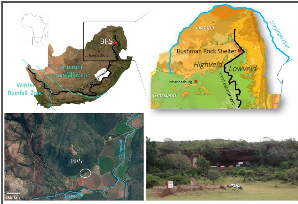
Figure 1: Location of Bushman Rock Shelter (BRS). Top left: map of South Africa with seasonal rainfall regimes and the Great escarpment. Top right: zoom on the Limpopo area with vegetation biomes (adapted from Mucina and Rutherford, 2006). Bottom left: aerial view of the site with major rivers. Bottom right: view of the south-facing shelter.
