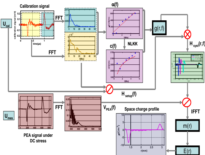
Fig. 2: Flow chart of the used deconvolution technique
