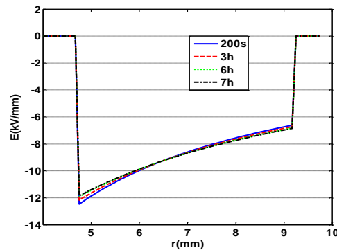
Fig. 5: Computed field distribution at different times in model cable stressed under -40kV at 22°C.
