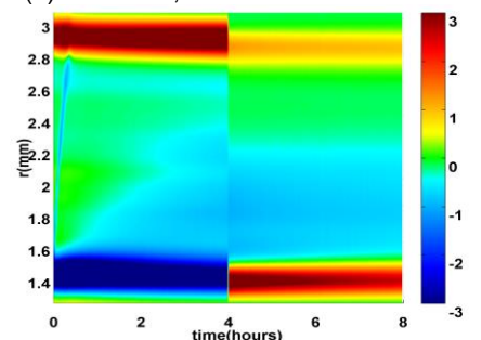
(b) Mini-cable, -55kV at temperature gradient
