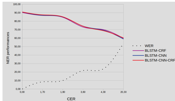
Fig. 1. NER F1-score degradation according character error rates
