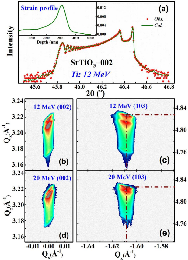
Figure 2. (a) The observed and calculated XRD profiles of the 12 MeV Ti ion irradiated SrTiO 3 around the Bragg peak (002). The maximum strain is \sim 1.32\% , and the corresponding depth dependent strain profiles are shown as inserts; (b) and (c) the reciprocal space maps of 12 MeV Ti ion irradiated sample around the (002) and (103) Bragg peaks; (d) and (e) the reciprocal space maps of 20 MeV Ti ion irradiated SrTiO 3 near the lattice point of (002) and (103).
