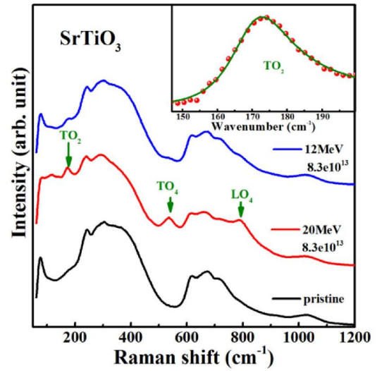
Figure 1. (a) The observed Raman spectrum of pristine SrTiO 3 and damaged with Ti ions of 12 MeV and 20 MeV in fluence of 8.3 \times 10^{13} ions cm -2 . (b) The fitting of the Fano asymmetric Raman modes TO 2 and TO 4 for the 20 MeV Ti ions irradiated sample. The Fano fitting parameters are A = 39.15 , q = 4.11 , \omega_0 = 170.2 cm -1 , and \Gamma = 21.98 cm -1 .
