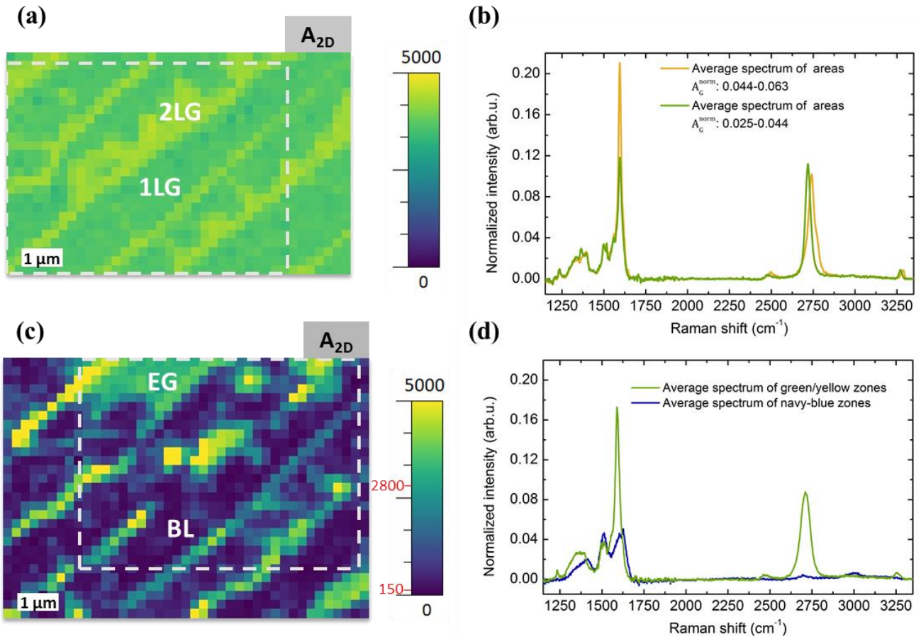
Figure 5: Raman analysis of a sample on which we have performed a graphene peeling. Two Raman A_{2D} maps (a) before and (c) after the graphene peeling (in \text{counts}\cdot\text{s}^{-1}\cdot\text{cm}^{-1} ). The dashed white rectangles mark the common area of these two maps. Different representative domains have been indicated as BL, 1LG, 2LG and EG. Figures (b) and (d) show the average spectrum of each domain. The scanning steps of both x and y directions are 0.25\ \mu\text{m}
