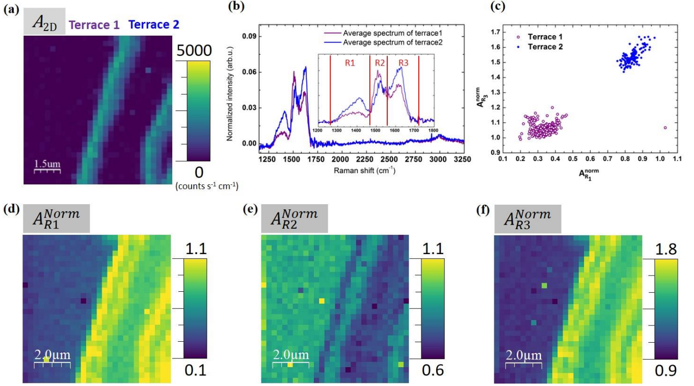
Figure 3: Raman analysis of sample DG1. (a) Raman A_{2D} map. Navy-blue areas correspond to BL_0 on two terraces, while green areas correspond to EG. (b) Average spectra of terrace 1 (purple) and terrace 2 (blue). Inset: zoom between 1200 and 1800 \text{cm}^{-1} . The vertical bars at 1260, 1460, 1550 and 1710 \text{cm}^{-1} delimit the 3 regions R1, R2 and R3 used in our analysis. (c) Relationship between A_{R_1}^{norm} and A_{R_3}^{norm} for the two terraces. (d-f) Raman A_{R_1}^{norm} , A_{R_2}^{norm} and A_{R_3}^{norm} maps.
