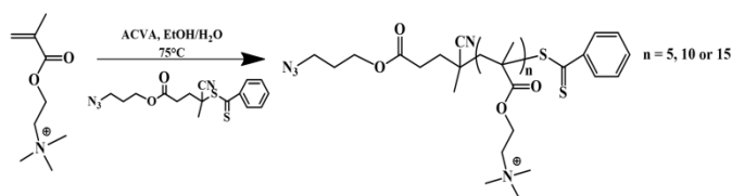
Scheme 1. Synthesis of cationic oligomers by RAFT polymerization of [2-(methacryloyloxy)ethyl]trimethylammonium chloride monomer
