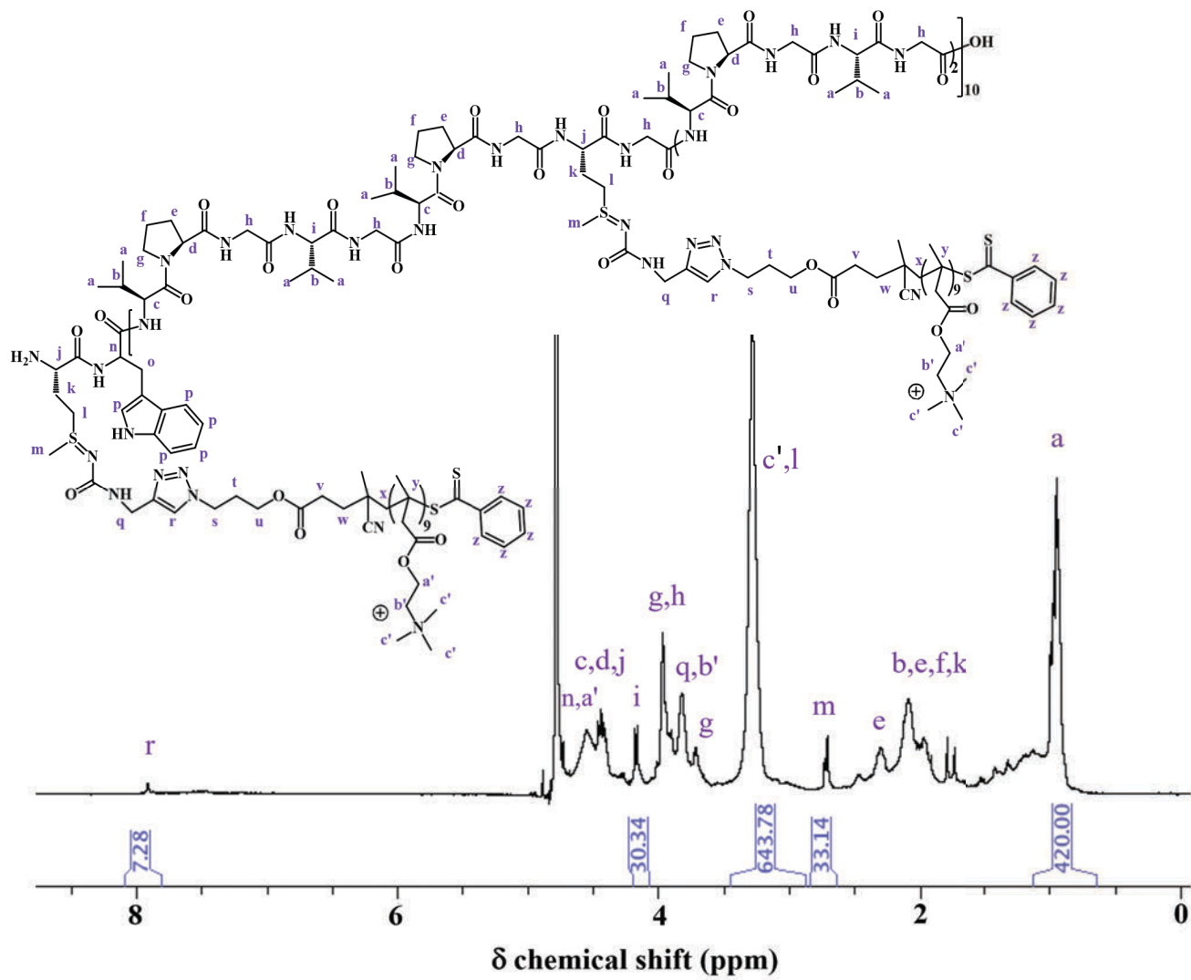
Figure S12.- 1 H-NMR spectra of ELP-g-P(TMAEMA) 9 in D 2 O (25 °C, 400.2 MHz).
