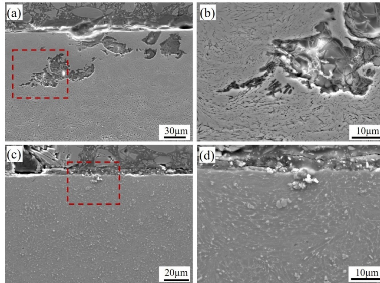
Fig. 8 SEM images showing the cross-sectional morphologies of the (a, b) 7075Al-C2 and (c, d) \text{TiB}_2 /7075Al-C2 deposits after 7 days immersion in 0.6 M NaCl solution.
