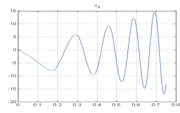
Fig. 9. Trajectory state of x_1 and x_2 respectively .
