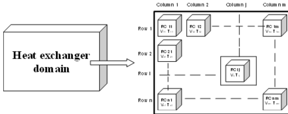
Fig. 2. Division of the heat exchanger domain into sub-domains (representative cells).
