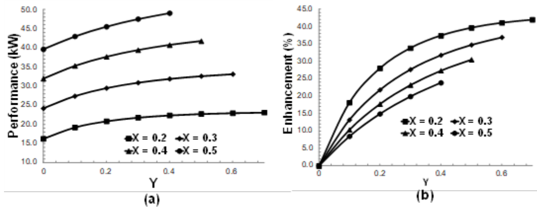
Fig. 4. Variation of the (a) HX thermal performance and (b) enhancement in function of X and Y.
