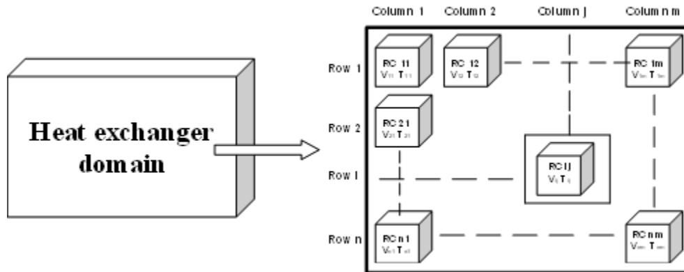
Fig. 2. Division of the heat exchanger domain into sub-domains (representative cells).
