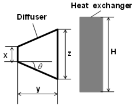
Fig. 3. Schematic including the parameters to be tested.
