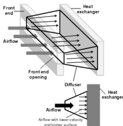
Fig. 1. New suggested design.
