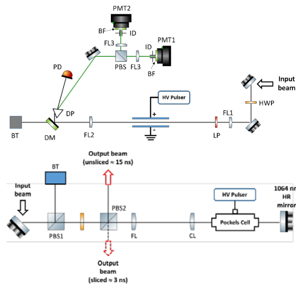
Fig. 1. (a) Experimental schematic for the E-FISH measurements. (b) Optical layout for the pulse slicer. (Legend – BF: bandpass filter, BT: beam trap, CL: plano-concave spherical lens, DM: dichroic mirror, DP: equilateral prism, FL: plano-convex spherical lens, HWP: half-wave waveplate, ID: iris, LP: longpass filter, PBS: polarizing beamsplitter, PD: photodiode, PMT: photomultiplier.)
