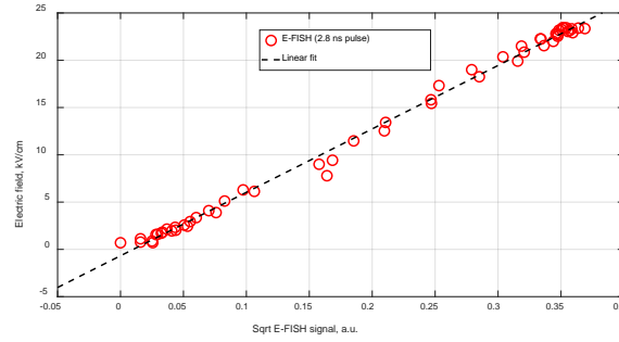
Fig. 2. (a) Time evolution of (square rooted) E-FISH signals produced by 2.8 ns pulses, appropriately scaled and plotted together with the field evolution measured by the back current shunt (BCS). The time-varying field is imposed by applying 30 ns (FWHM) HV pulses with a rise time of about 8 ns. (b) Calibration curve obtained by plotting the measured field values from the BCS against the square root of the E-FISH signals. All acquired signals are averaged over 300 laser shots.
