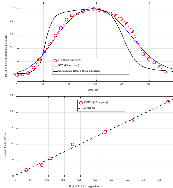
Fig. 3 (a) Comparison of the peak-normalized electric field evolution measured by the BCS versus the peak-normalized E-FISH signal evolution, using 16 ns pulses. (b) Peak applied field strength as a function of the square root of the E-FISH signal.
