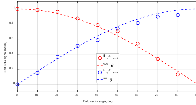
Fig. 4 Horizontal ( x ) and vertical ( y ) components of the peak-normalized, square-rooted E-FISH signals as a function of the field vector angle, \theta . For a given angle \theta , the horizontal and vertical components of an applied field E_{ext} vary as E_{ext} \cos \theta and E_{ext} \sin \theta , respectively.
