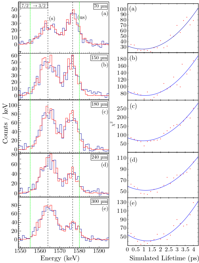
Figure 4. (Color online) Left: Comparison of fits of the simulated GEANT4 \gamma -ray 7/2^- \rightarrow 3/2^-_{\text{g.s.}} transition (red) and measured spectra (blue) at five distances (a-e) used for the lifetime determination. The vertical black dashed lines mark the shifted (s) and unshifted (us) components after Doppler correction for the degraded component, the green dashed lines mark the area used for calculation of the \chi^2 values. Right: Reduced \chi^2 values (red dots) versus simulated lifetime with a best fitting of the quadratic function (blue line) for each distance. See text for details.
