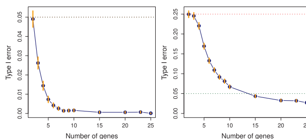
Fig. 1. Evolution of type I error of detecting two completely disjoint groups of RNAs with the number of RNA in the experiment, for individual tests of ratio changes with P_{i,i'} < 0.05 (left) or P_{i,i'} < 0.25 (right). Upper line: individual tests level \alpha_0 ; lower dotted line: P = 0.05 . Vertical segments are \sim 95\% confidence intervals of the type I error estimated from 10 000 simulations
