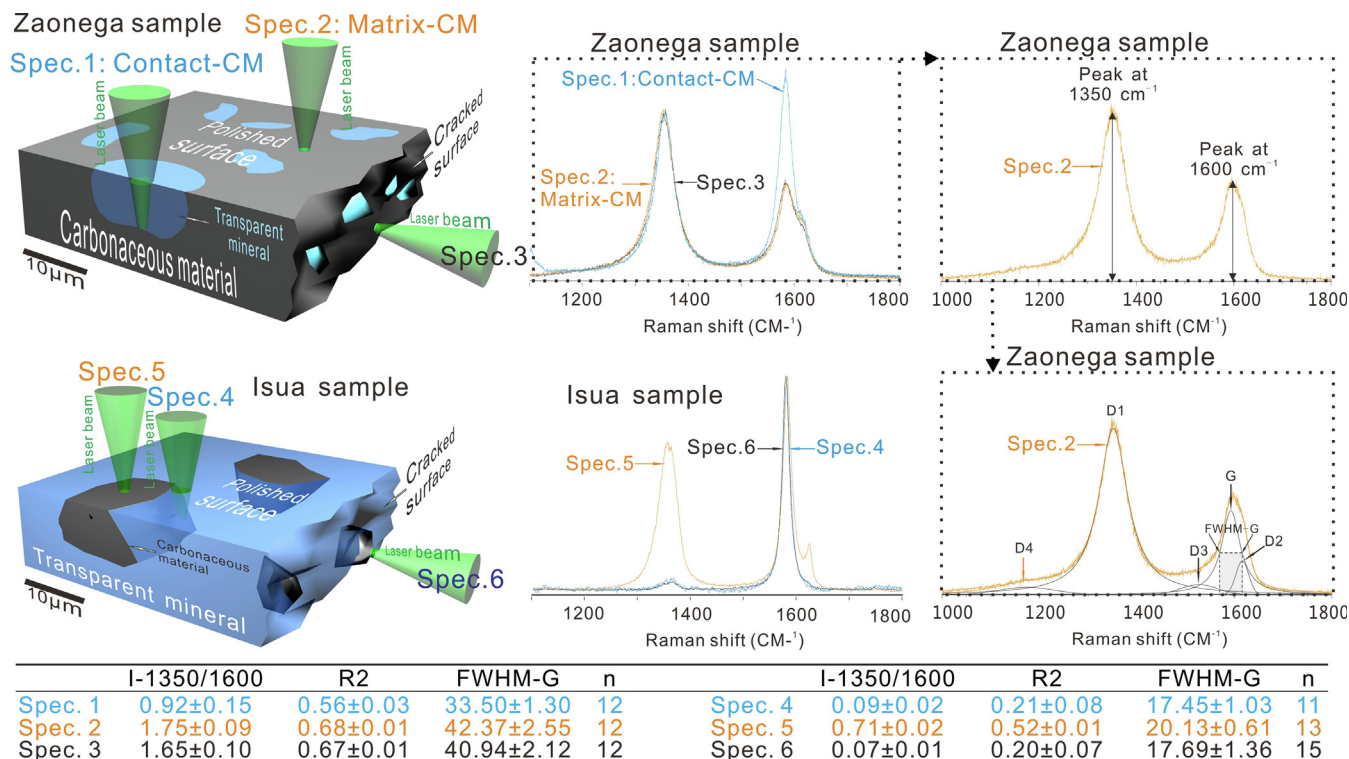
Fig. 3. Test of polishing and cracking artifacts on the structure of CM: A specific comparison is made here between a sample from the organic-rich part at 413 m depth of drill core 12AB of the Zaonega Formation, and a graphite-bearing metacarbonate from the 3.7 Ga Isua Supracrustal Belt, Western Greenland (amphibolite-facies metamorphism). Representative Raman spectra obtained at specific locations are: for the Zaonega Formation Spec. 1 Contact-CM at the subsurface, Spec. 2 Matrix-CM at the polished surface, Spec. 3 Matrix-CM at the freshly cracked surface; for the Isua Supracrustal Belt Spec. 4 Graphite at the subsurface, Spec. 5 Graphite at the polished surface, Spec. 6 Graphite at the freshly cracked surface. Listed below this are the average values of I-1350/1600, R2 and FWHM-G, standard deviations and measured numbers. In the dashed box, a representative Raman spectrum illustrates two different ways of deconvoluting the spectrum used in this study: 1) defining I-1350/1600 as the intensity ratio of peaks at 1350 cm -1 and 1600 cm -1 ; 2) decomposing the spectrum into D1-, D2-, D3-, D4- and G-peaks, and calculating the parameter R2 = D1/(G + D1 + D2) and FWHM-G = full width at half maximum of the G-peak.
