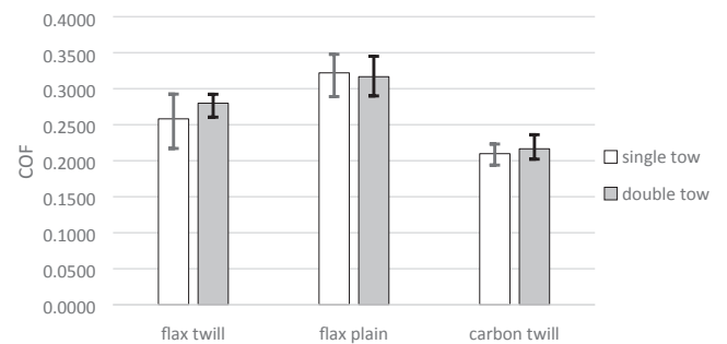
Fig. 10. Average friction coefficient for single and double tow setups at 0° shear (the error bars represent min and max values in each configuration).
