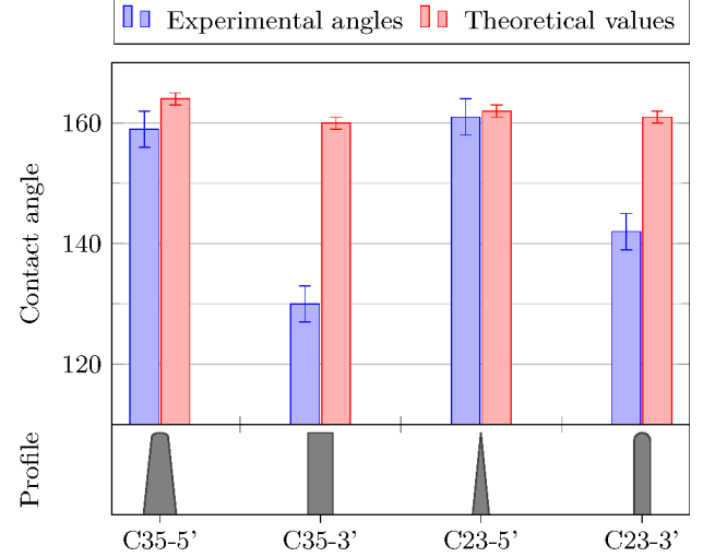
FIG. 4. (Color online). Comparison for each kind of patterns between experimental (blue) contact angles (in degrees) and theoretical ones (red) from Eq. 10 assuming quantum contributions inducing superhydrophobicity. The patterns are classified according to two extreme shapes, i.e. pillars (cylinders) and spikes (sharp cones).
