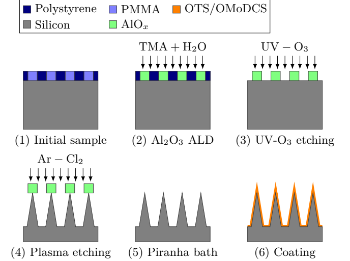
FIG. 2. (Color online). Sketch of each fabrication step 1 to 6 detailed in the text. 1. Formation of honeycomb structure of PMMA self-assembled studs in a PS matrix using block copolymer nano-manufacturing. 2. PMMA domain conversion into \text{Al}_x\text{O}_y (green) by sequential infiltration synthesis. 3. Selective removal of the PS matrix using UV- \text{O}_3 treatment. 4. Silicon etching by RIE with \text{Al}_x\text{O}_y nanostructures as hard mask. 5. Hard mask stripping. 6. Organosilane monolayer grafting.
