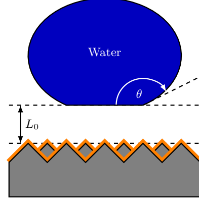
FIG. 1. (Color online). Sketch of the studied system. At equilibrium, the water droplet is separated from the nanostructured surface by the distance L_0 16 . The droplet presents a contact angle \theta . The nanostructured silicon (grey) is coated (orange) with organic molecules in order to emulate a nanostructured molecular solid surface.
