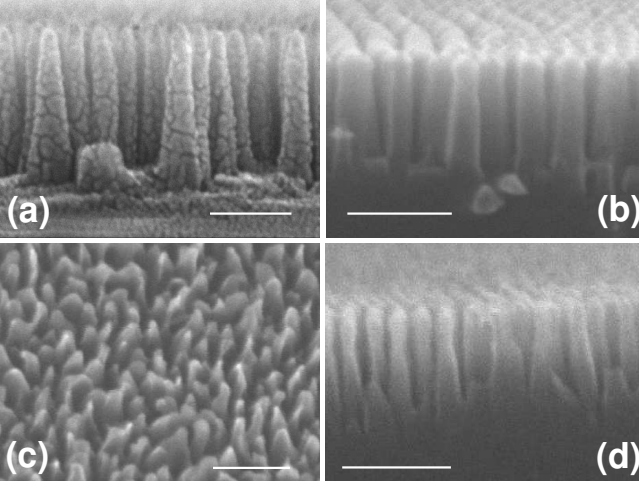
FIG. 3. Scanning electron microscopy images of nanopatterned silicon surfaces for C35-5' sample (a), C35-3' sample (b), C23-5' sample (c) and C23-3' sample (d). Scale bar: 100 nm.
