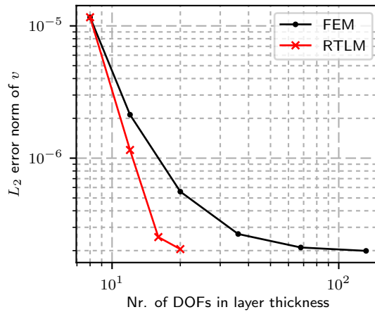
Figure 9: Convergence of the two methods with fixed element widths, based on L_2 error norm of the top surface vertical displacement and the number of dofs stacked on a single underlying node position. Simulation with 160 elements underlying the surface layer in the contact region and \nu = 0.49 .
