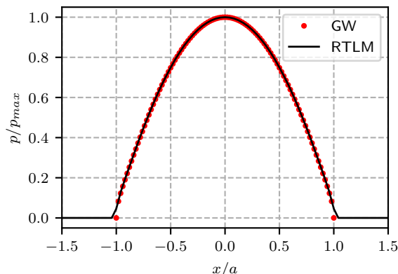
Figure 13: Comparison of the resulting pressure distribution for Greenwood solution (GW) and RTLM contact simulation implemented in ABAQUS. (Indenter of shape \phi = x^2/2R , where R = 50 and a/e = 5 .)
