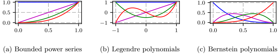
Figure 12: Illustration of different polynomial bases for cubic expansion.
