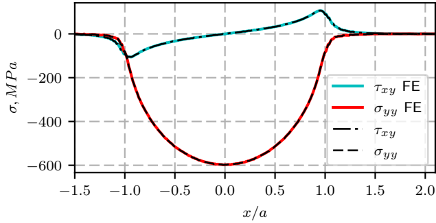
(b) Stress along \Gamma(\hat{y} = 0) (coating substrate interface)
