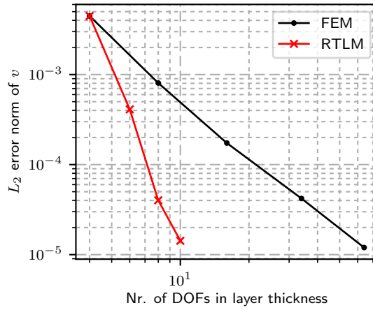
Figure 8: Convergence of the two methods with fixed element widths, based on L_2 error norm of the top surface vertical displacement and the number of dofs stacked on an underlying node position. Simulation with 500 elements underlying the surface layer in the contact halfwidth and \nu = 0.49 .
