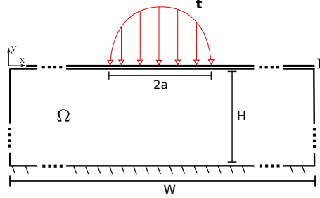
Figure 3: Illustration of the "semi-infinite" domain considered for the numerical analysis. Dimensions of the domain are considered to be large, a/H = a/W \ll 1 . For illustration purposes the sides are shortened by usage of the symbol "...".
