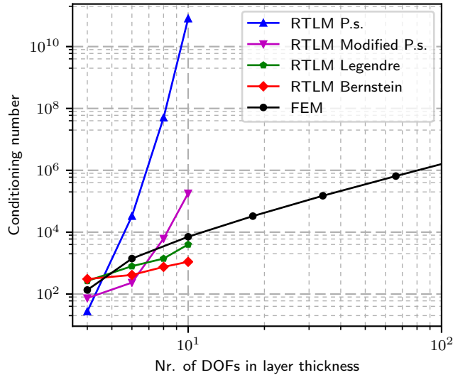
Figure 11: Conditioning number dependency on number of dofs for different polynomial expansion basis.
