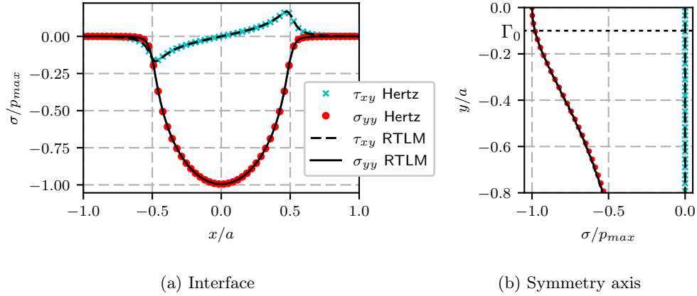
Figure 6: Shear and compressive stresses along a) interface \Gamma(\hat{y} = 0) and b) symmetry axis ( x=0 ), with parameters E_s = E_c = 200 GPa, \nu = 0.4 , p = 3 , a/e = 10 .
