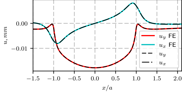
(a) Displacements along \Gamma(\hat{y} = e) (top surface)
