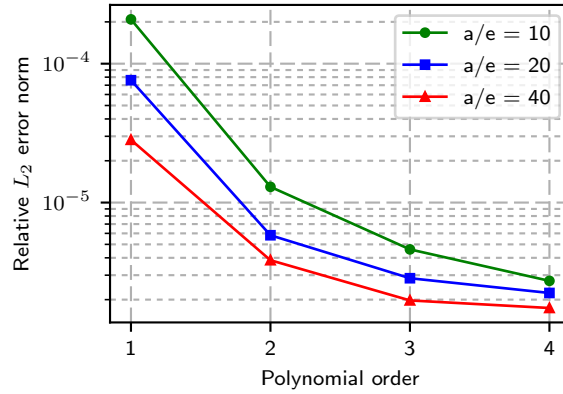
Figure 4: Relative L_2 error norm over \Gamma(\hat{y} = e) for top surface displacement v(x, y = e) according to polynomial order. Used model parameters are E_c = 0.6 GPa, \nu = 0.4 and ratio of the contact half-width and the layer thickness is noted as a/e .
