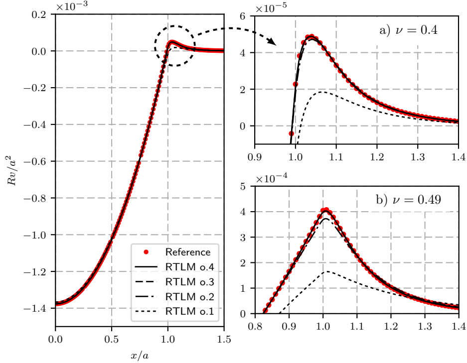
Figure 5: "Pile-up" capture according to polynomial order used. (Results for cases with a/e = 20 , R/a^2 = 200 , where shape of indenter is defined as \phi = x^2/2R .) Main figure displays the shape of the indentation, whereas a) and b) display close-up views of the "pile-up" region with different Poisson ratio values.
