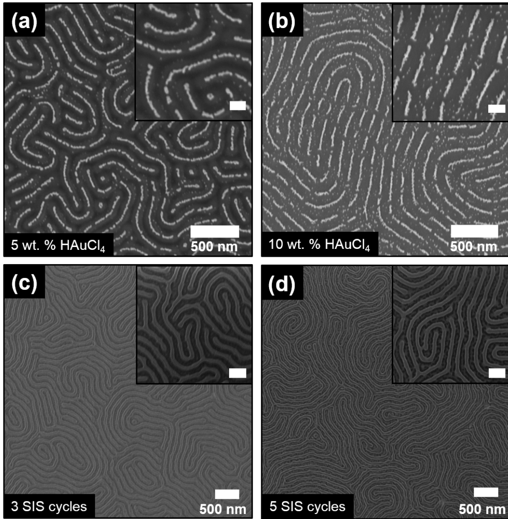
Figure 5. Large period metallic and dielectric feature formation. (a,b) Top-down SEM images showing Au metallic features from 5 wt. % and 10 wt. % \text{HAuCl}_4 solutions deposited on PSPVP3 templates and treated with \text{O}_2 plasma. Insets show high-resolution images of defined Au features, scale bars are 100 nm. (c,d) Top-down SEM images showing \text{AlO}_x feature formation after SIS treatment for 3 cycles and 5 cycles respectively. Insets show high-resolution images of \text{AlO}_x features, scale bars are 200 nm. Periods in all images are \approx 110 nm.
