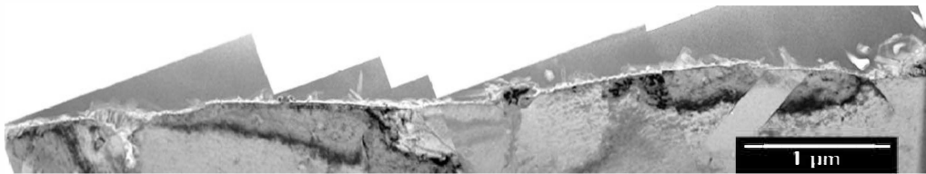
Figure 17. TEM bright field images of the oxide developed on the inner extreme surface of the steam generator tube in alloy 690 exposed in primary water during transients test until 325°C
