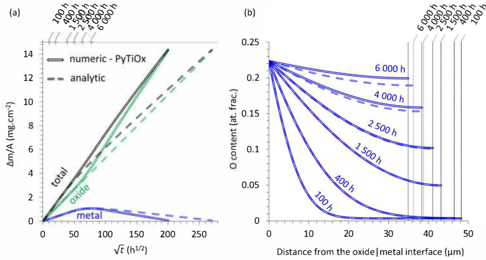
Fig. 7. Comparison of the evolution of numerically and analytically (Fig. 5) calculated mass gains as a function of the square root of time for a 100 \mu\text{m} thick sample using Pawel's and PyTiOx models for 73 000 h of oxidation at 650 ^{\circ}\text{C} (a) and evolution of the O diffusion profiles within the metallic matrix (progressively consumed by the oxide growth) relative to a 100 \mu\text{m} thick sample (b).
