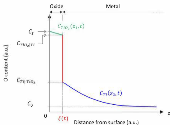
Fig. 15. Graphical illustration of Wagner's model.
