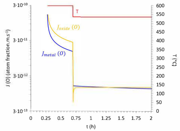
Fig. 12. Evolution of oxygen fluxes getting out of the oxide (orange) and getting into the metal (blue) as a function of time during the temperature transient from 600 °C to 535 °C. (For interpretation of the references to colour in this figure legend, the reader is referred to the web version of this article.)
