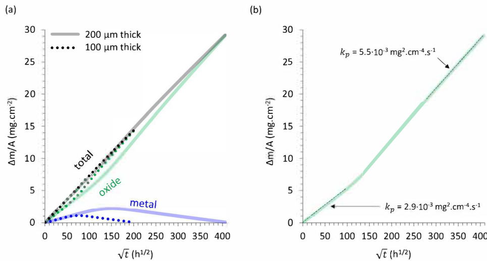
Fig. 8. Overlay of the calculated mass gains per unit area using the PyTiOx model for the oxidation of two different sample sizes (100 \mu\text{m} and 200 \mu\text{m} thick) at 650 ^{\circ}\text{C} (a) and focus on the two successive parabolic regimes forming the oxide growth kinetics curve (b).
