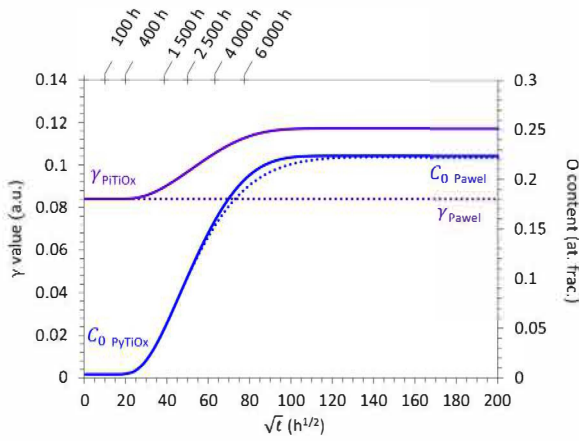
Fig. 9. Evolution of \gamma and C_0 over time calculated from Pawel's and PyTiOx models for a 100 \mu\text{m} thick sample.
