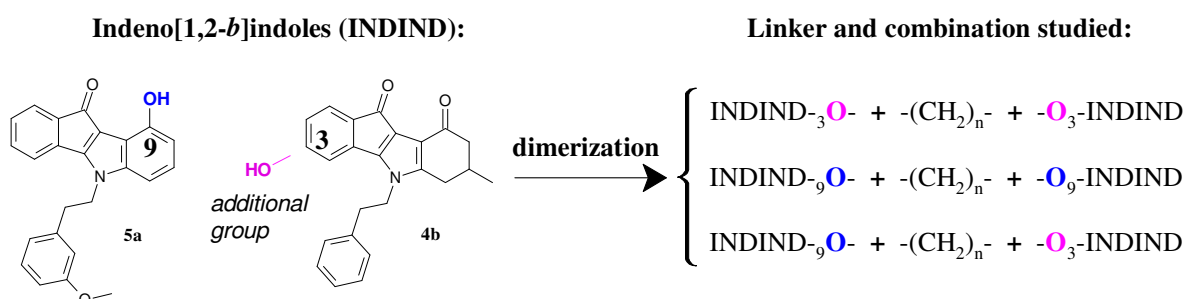
Fig. 2. Chemical structures of monomeric indeno[1,2- b ]indoles 4b , 5a and modulation sites for dimerization (OH groups used for dimerization are shown in blue and magenta, linker length (n) varied between 2 and 12 carbons).
