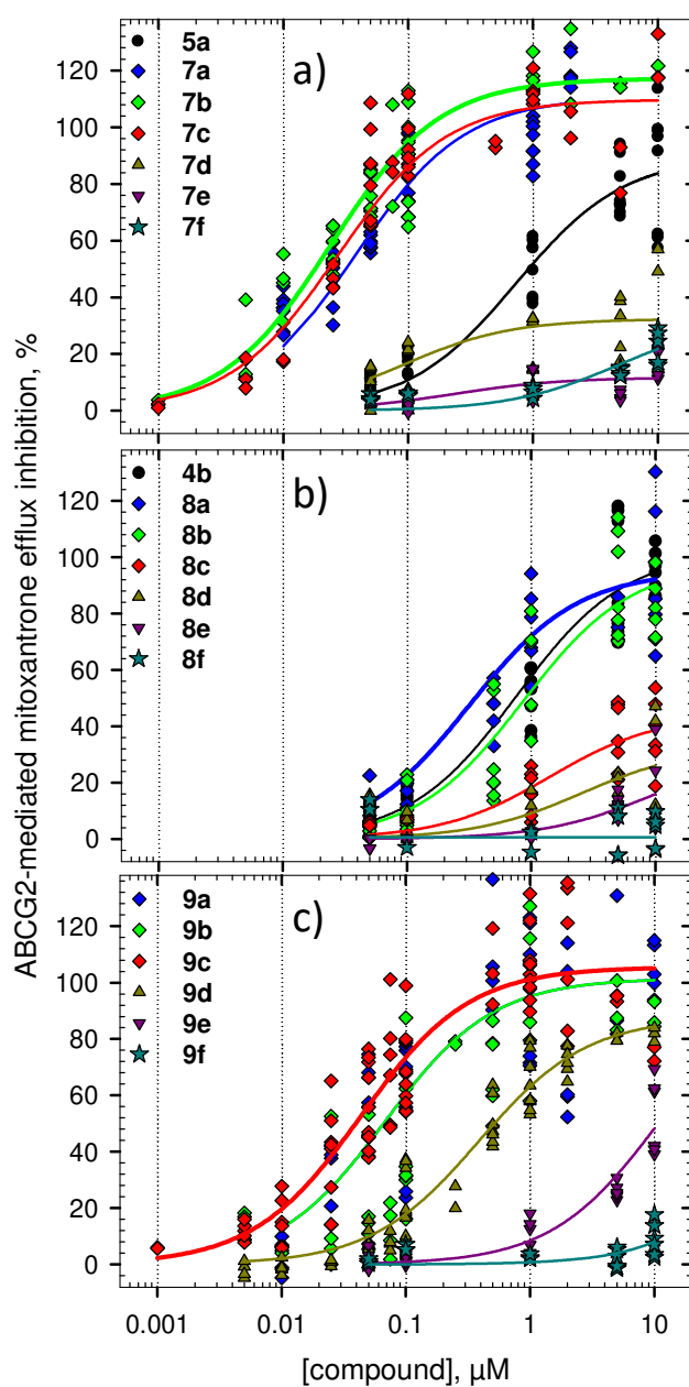
Fig. 3. Evaluation of the inhibitory efficacy of the ABCG2-mediated mitoxantrone efflux by dimers and parent compounds. HEK293-ABCG2 cells were incubated with 5 \mu M
