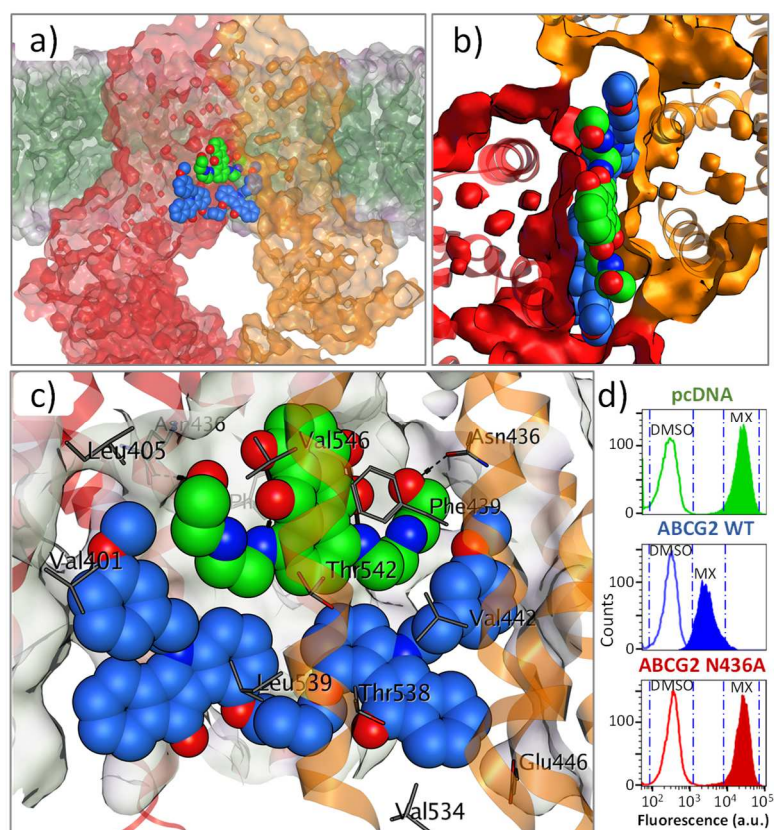
Fig. 5. Molecular docking of 7b (blue) and mitoxantrone (green) into the cryo-EM structure of ABCG2. a-c) ABCG2 (PDB 5NJ3 [7], red + orange) after dynamic simulation with lipids (pale green). Close residues are labelled. d) Flow cytometry analysis of mitoxantrone (MX) intracellular fluorescence accumulation in control HEK293 cells (pcDNA) or expressing WT or N436A versions of ABCG2, and DMSO as control.
