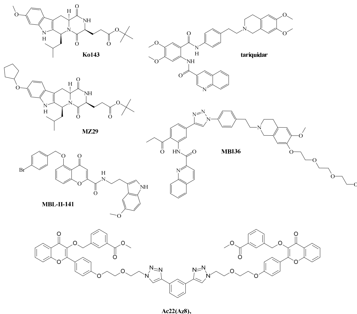
Fig. 1. Chemical structures of Ko143, MZ29, tariquidar, MB136, MBL-II-141 and Ac22(Az8) 2 .
