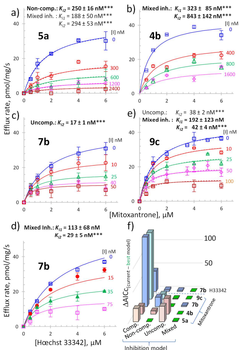
Fig. 4. Inhibition mechanisms by 4b , 5a , 7b and 9c . a-e) ABCG2-mediated mitoxantrone or Hoechst 33342 efflux rates plotted with respect to substrate and inhibitor concentrations, corresponding to the residual intracellular substrate amounts in HEK293- ABCG2 vs HEK293. Best and close models are displayed with their inhibitor constant (in bold for the best model). Data set ranging from 72 to 204 points were from 1 (d), 2 (a, b), 3 (e) or 5 (c) experiments done in duplicates (c, e) or triplicates (a, b, d). *** p < 0.001 . f) Ranking of inhibition models using their AICc. The difference of a given AICc with the lowest found corresponding to the best model is plotted. Best and close models are colored in green (Fig. S5-8).
