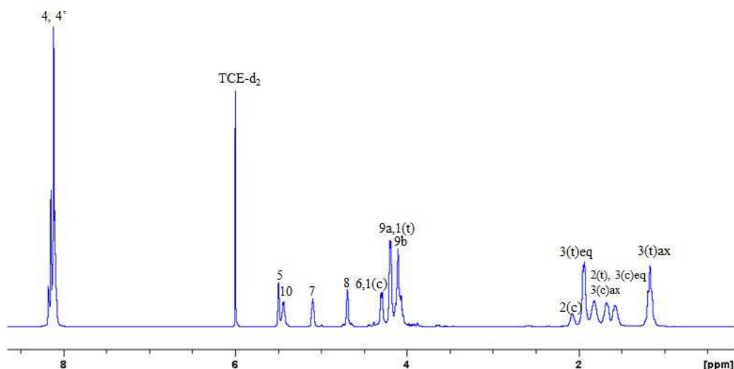
Figure 3. ^1\text{H-NMR} spectrum of \text{PCI}_{40}\text{T} with peak assignments ( \text{C}_2\text{D}_2\text{Cl}_4 at 25\text{ }^\circ\text{C} , 400\text{MHz} ).
