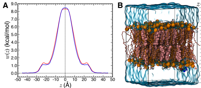
FIG. 13. Potential of mean force characterizing the permeation of a 1-palmitoyl-2-oleoyl-phosphatidylcholine:cholesterol membrane by 2',3'-dideoxyadenosine, obtained using ABF (red line) and meta-eABF (blue line) (A). The reaction-coordinate model is the projection onto the z -axis of the distance separating the center of mass of the permeant from that of the lipid bilayer (B).
