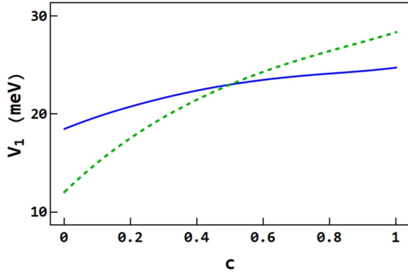
Figure 2. Evolution of the nearest-neighbor effective pair interaction V_1 with the concentration c when the curvature of the site energies is not taken into account V_1^{\text{sing}} (blue) and when it is V_1^X (green, dashed).
