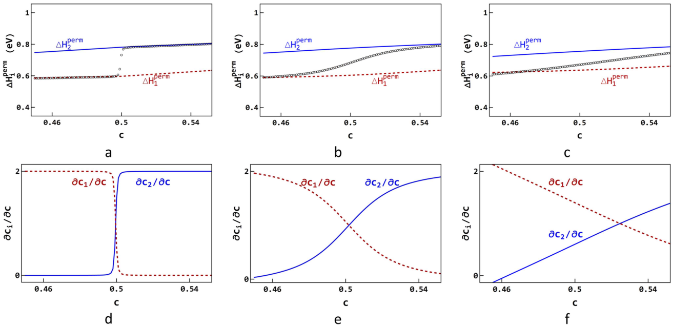
Figure 7. Permutation enthalpy of the 2 sublattices and of the total system in the concentration range of the L1 0 structure (a–c). Evolution of dc_i/dc with the concentration for the 2 sublattices (d–f). T = 150 K (a, d), T = 300 K (b, e) and T = 450 K (c, f).
