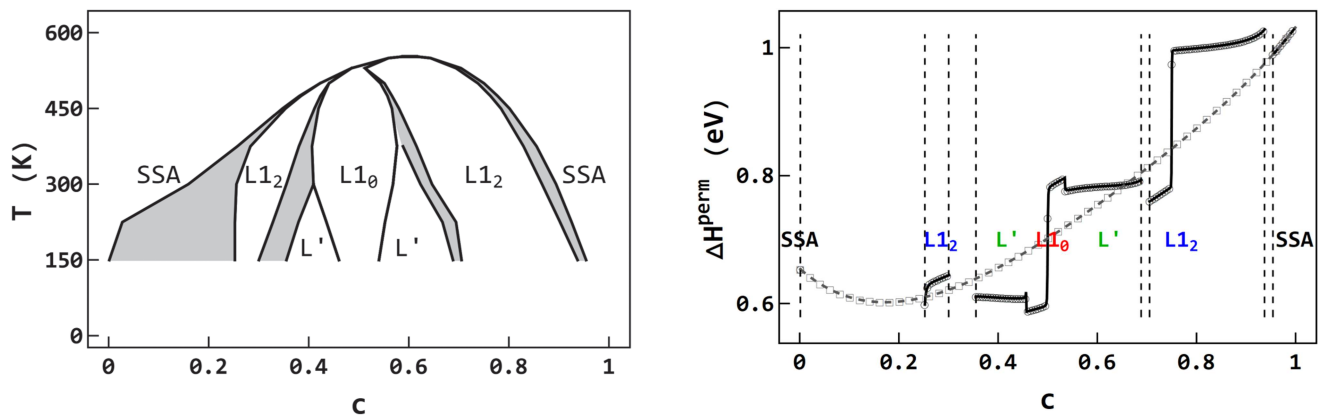
Figure 5. Comparison of \Delta H^{\text{perm}}(c) of LRO ( T = 150 K) (continuous lines) and of RSS ( T = 1000 K) (dashed) with also a comparison with direct calculation (symbols).
