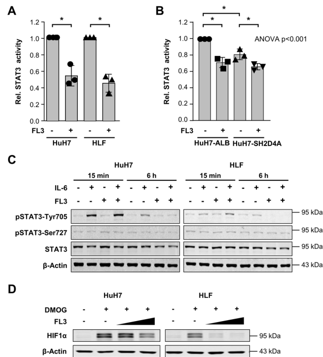
Fig. 4 FL3 reduces IL-6-induced STAT3 transcriptional activity and inhibits induction of HIF1α. A Luciferase assay of HuH7 and HLF cells measuring endogenous STAT3 transcriptional activity using STAT3 binding elements upon treatment with 20 ng/mL IL-6 in the absence or presence of FL3 (100 nM) for 6 h. Renilla luciferase was used as an internal transfection control and for normalization. Data were normalized to corresponding IL-6 stimulated control cells. *p < 0.05 . B To test the effect of SH2D4A on STAT3 transcriptional activity, HuH7 cells infected with pTRIPZ-SH2D4A or pTRIPZ-ALB as control and treated with doxycycline (DOX) 1 day after transfection of Luciferase and Renilla reporter constructs. Luciferase activity upon treatment with 20 ng/mL IL-6 in the absence or presence of FL3 (100 nM) for 6 h was measured. Data are represented as mean \pm SD of three independent experiments with each data point representing the mean of two technical replicates within each experiment. *p < 0.05 for pairwise comparison and ANOVA test was performed on the three mean values of independent experiments comparing all four groups. C Western blots of HuH7 and HLF cells upon stimulation with 20 ng/mL IL-6 or/and FL3 (100 nM) for 15 min or 6 h, as indicated. D FL3 reduced DMOG-induced HIF1α protein level dose-dependently. Cells were stimulated with 1 \mu M DMOG and FL3 in two different concentrations (50 nM and 100 nM) for 4 h.
