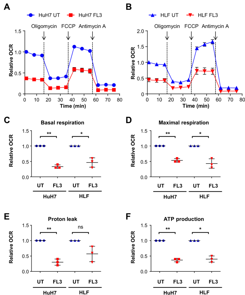
Fig. 6 Mitochondrial respiration is impaired by FL3 treatment. A Cells were treated with 100 nM FL3 for 24 h or left untreated as control (UT). The oxygen consumption rate (OCR) was measured with the Seahorse XF96 Analyzer in HuH7 and B HLF cells applying mitochondrial stress test conditions. Results of three independent experiments are expressed as mean \pm SEM. FCCP: Carbonyl cyanide-4-(trifluoromethoxy)phenylhydrazone. C Basal respiration, D maximal respiration, E proton leak, and F ATP production were measured and calculated for HuH7 and HLF cells. Mean data points from three independent experiments are depicted in scatter plots with mean \pm SD. * p < 0.05 , ** p < 0.01 , ns: not significant for pairwise comparison.
