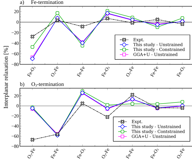
FIG. 3. Interplanar relaxations [in %] for unstrained and constrained Fe- and O 3 -terminated \alpha -Fe 2 O 3 (0001) surfaces in comparison with previous experimental 19,20 and theoretical 24 investigations.
