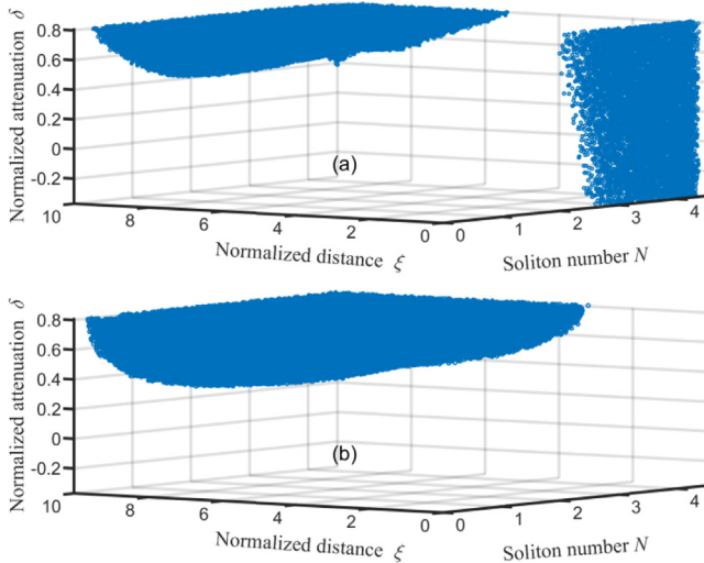
Fig. 5. Regions in the three-dimensional space ( N , \xi , \delta ) that enable the formation of a parabolic intensity profile (characterized by an excess kurtosis value between -0.9 and -0.8 ) in the (a) temporal and (b) spectral domains, as obtained from the NN model.
