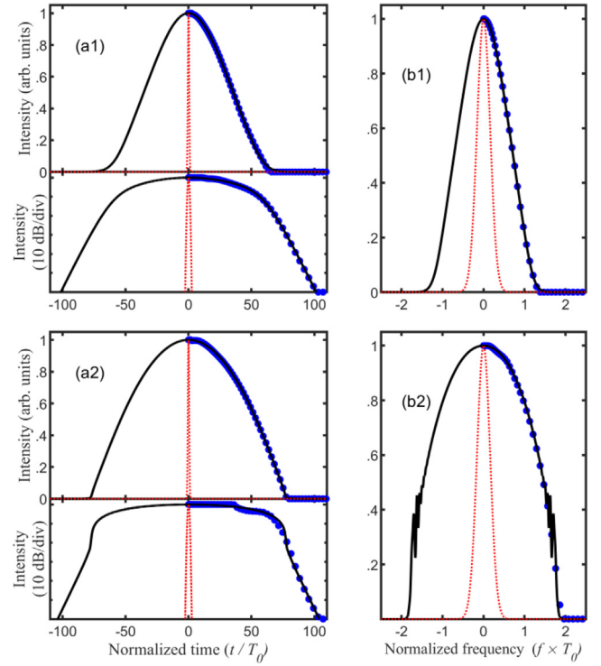
Fig. 2. (a) Temporal and (b) spectral intensity profiles of an initial Gaussian pulse after propagation in a lossy/gain normally dispersive fibre with \xi = 8 , N = 4 and \delta = -0.23 (panels 1) or \delta = 0.69 (panels 2). The predictions from the NN algorithm (blue circles) are compared with the results of NLSE numerical simulations (black curves). Also shown are the input intensity profiles (red dotted curves). The temporal profiles predicted by a second NN are displayed in the bottom parts of panels a using a logarithmic scale. (For interpretation of the references to color in this figure legend, the reader is referred to the web version of this article.)
