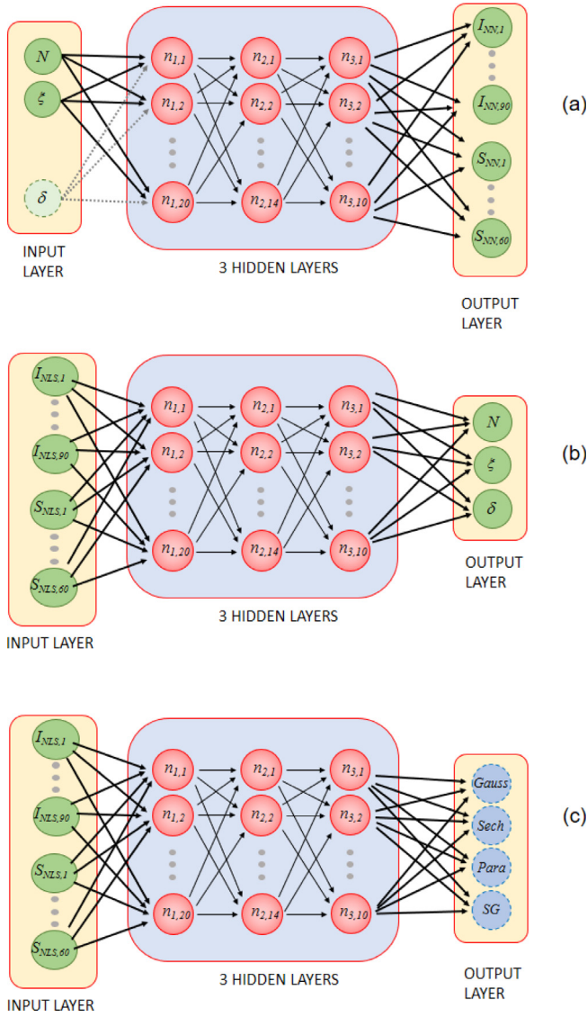
Fig. 1. NN model used to: (a) predict the output pulse intensity profiles from the fibre, (b) retrieve the nonlinear propagation properties and (c) identify the input pulse waveform.
