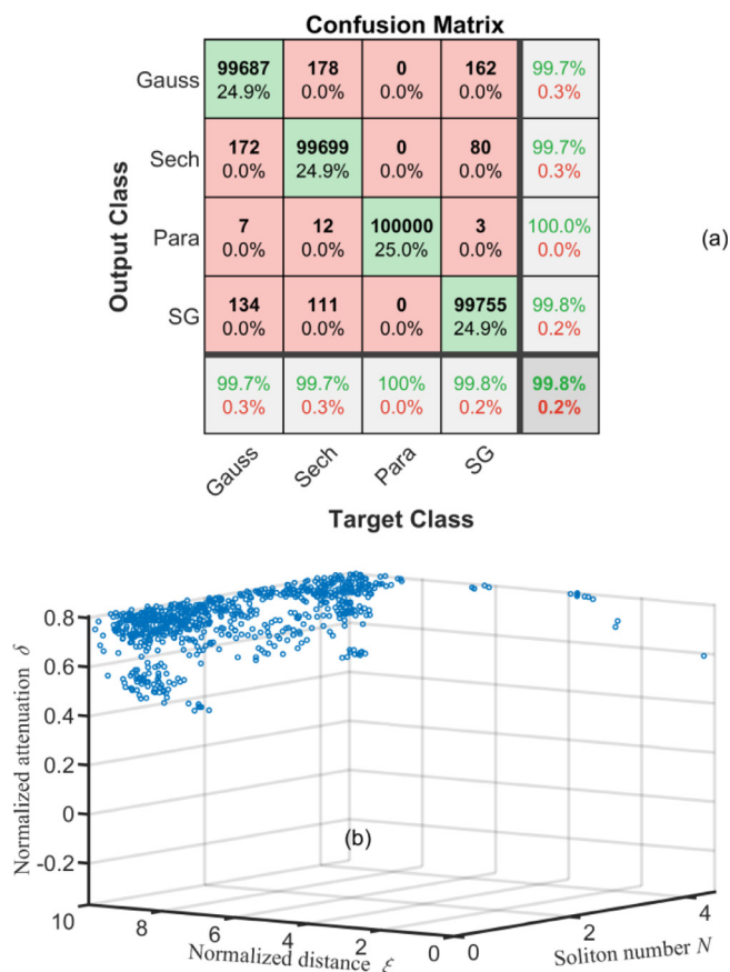
Fig. 9. (a) Confusion matrix relating to the initial pulse shape when the NN is interrogated with randomly chosen new simulated output pulses from the fibre corresponding to an unlabeled mix of input Gaussian, hyperbolic secant, parabolic and super-Gaussian pulses. (b) Points where prediction errors occur in the three-dimensional space (N, \xi, \delta) .
