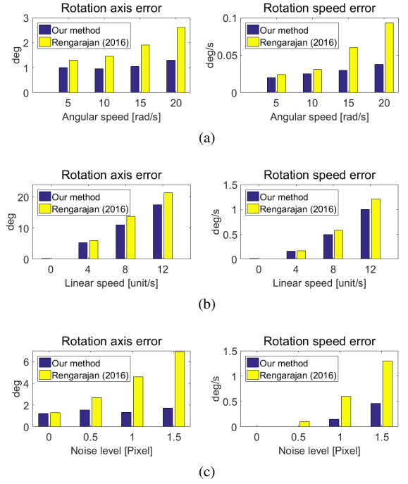
Fig. 5: Evaluation of ego-rotation computation: (a) effects of an increasing angular velocity. (b) Effects of an increasing translational velocity. (c) Effects of image noise level.
