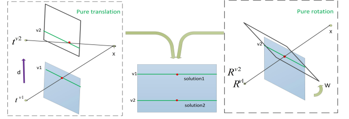
Fig. 3: Two examples of double-projections pattern. On the left, a RS camera is under pure translation heading to [0; 1; 0]^T rapidly. Besides, an example of pure-rotation with axis (1, 0, 0) shown on the right. A 3D point \mathbf{X} will be observed twice at row v_1 and v_2 if the speeds are big enough.
