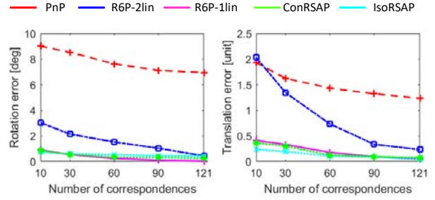
Fig. 16: AP errors for IsoRSAP , ConRSAP , PnP , R6P-2lin and R6P-1lin under different number of correspondences.
