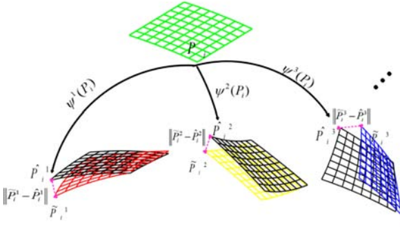
Fig. 11: 3D-3D RS registration recovers the actual shape \mathbf{P}_i (green) by minimizing the sum of squares of the distance between re-deformed shapes (black) \Psi^j(\mathbf{P}_i) and the equivalent RS deformed shapes \hat{\mathbf{P}}_i^j (red, yellow and blue) recovered by NRSfM.
