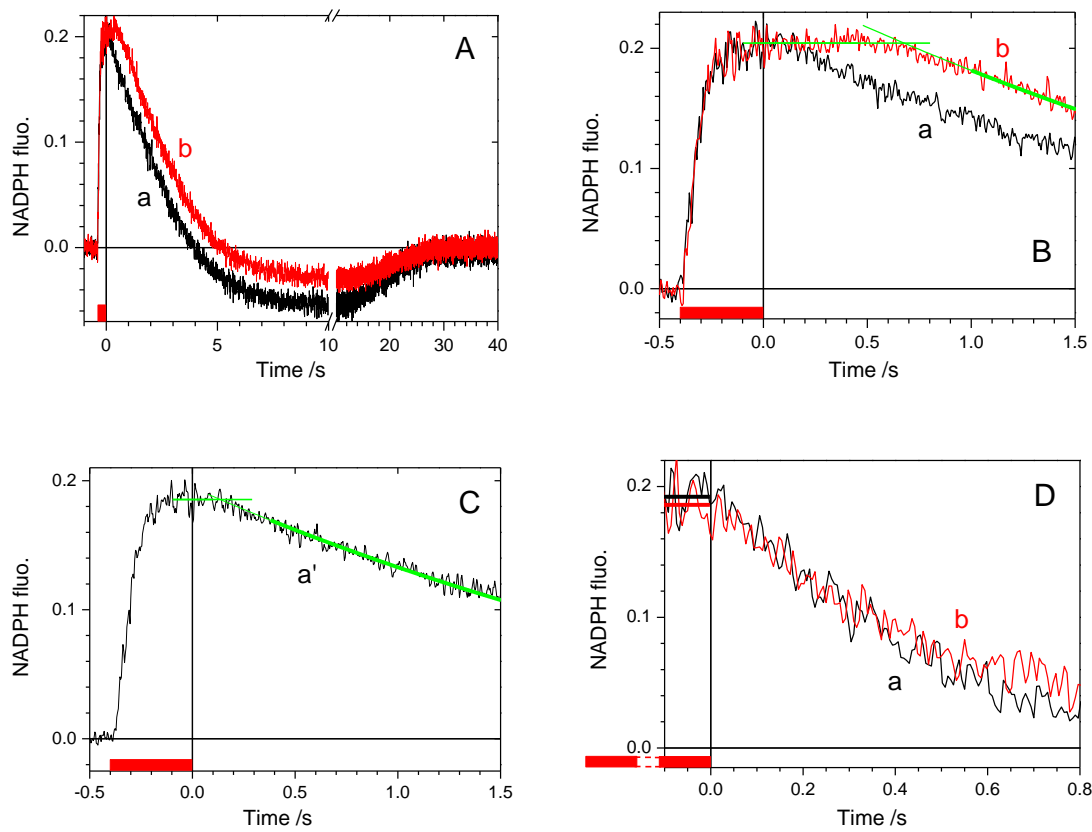
Fig. 1. NADPH fluorescence kinetics in WT and \Delta flv1/3 cells.
