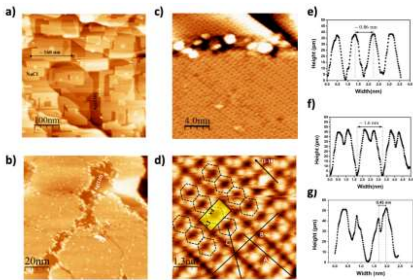
Figure 2: Occupied-state STM images corresponding to (a) 1ML NaCl film on Ag(110) ( 500 \times 500 \text{ nm}^2 , U = -1.05 \text{ V} , I = 0.7 \text{ nA} ), (b) 1 ML of silicon deposited over the NaCl film ( 100 \times 100 \text{ nm}^2 , U = -1 \text{ V} ,
